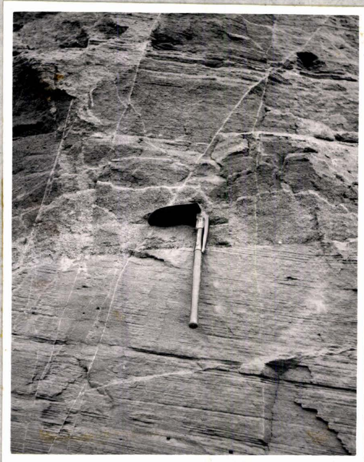
Fig. 16.- Tilted stratified quartz sand overlain by coarse shale sands.
