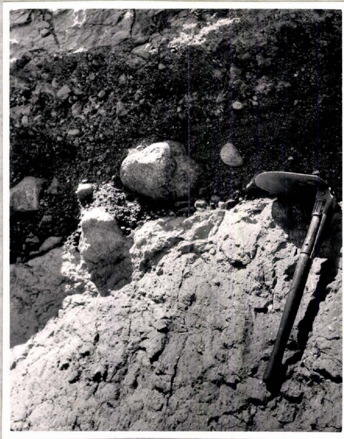
Fig. 12.- Close-up view of boulder pavement.
