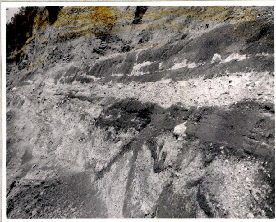
Fig. 13.- Folding in upper till caused by solifluction. Wave length of folds averages 6 feet.
