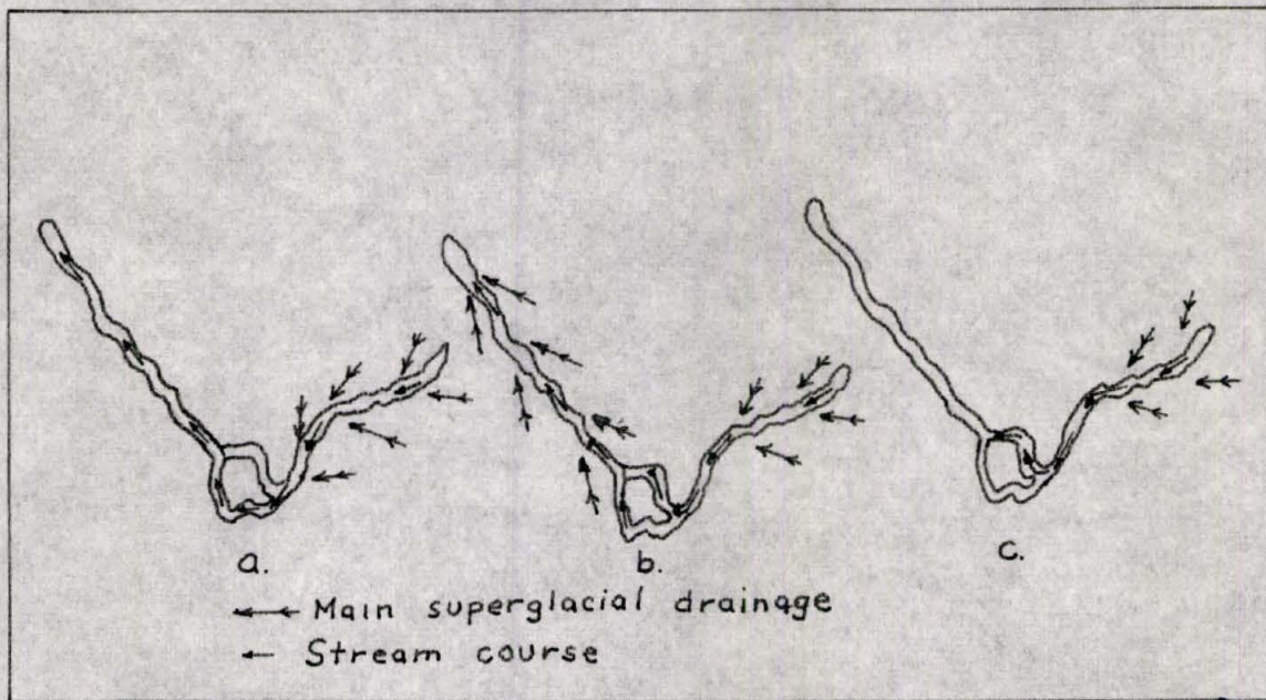
Fig. 4. Order of development of esker.
