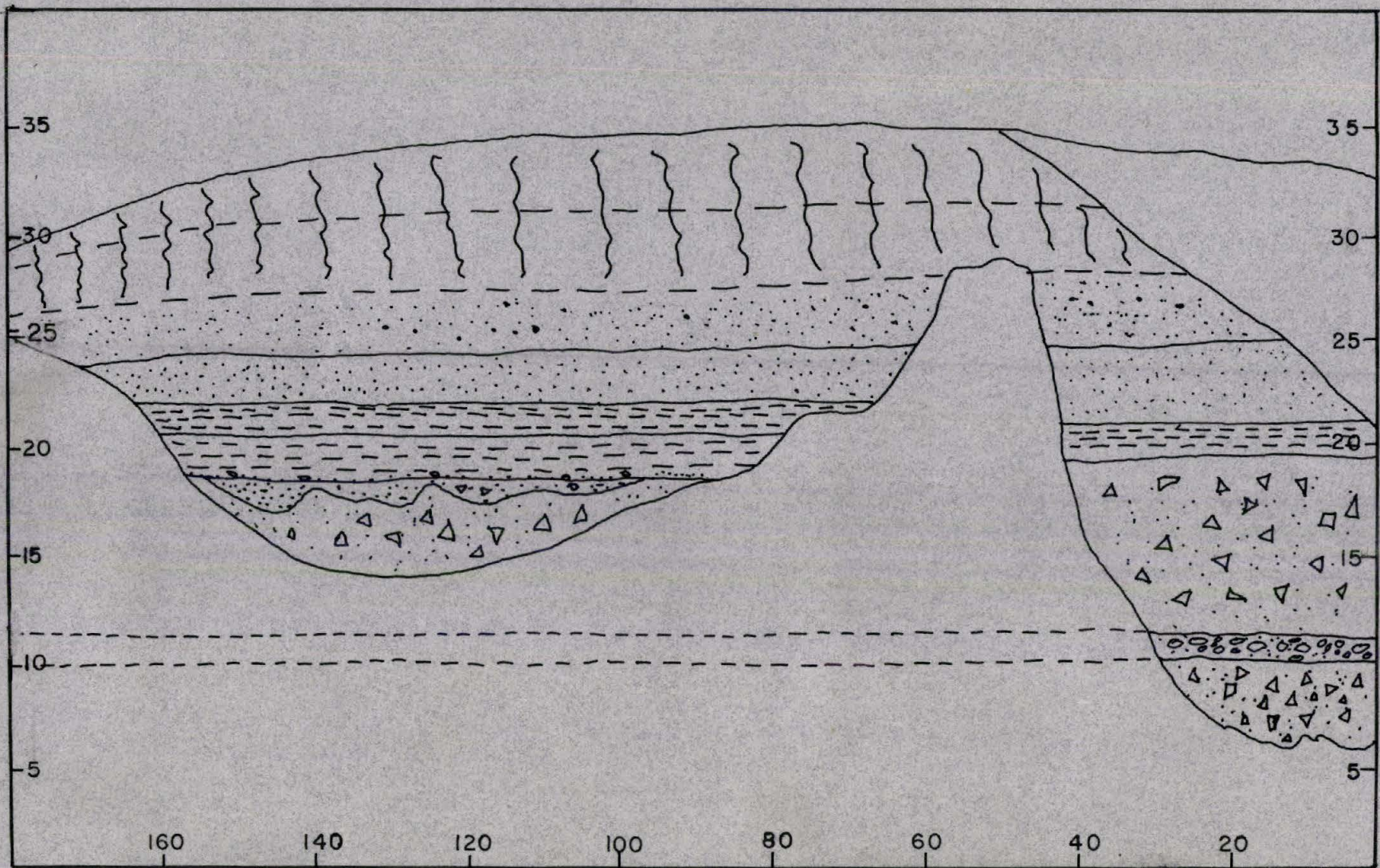
Fig 8 - Cross section of Park River site
