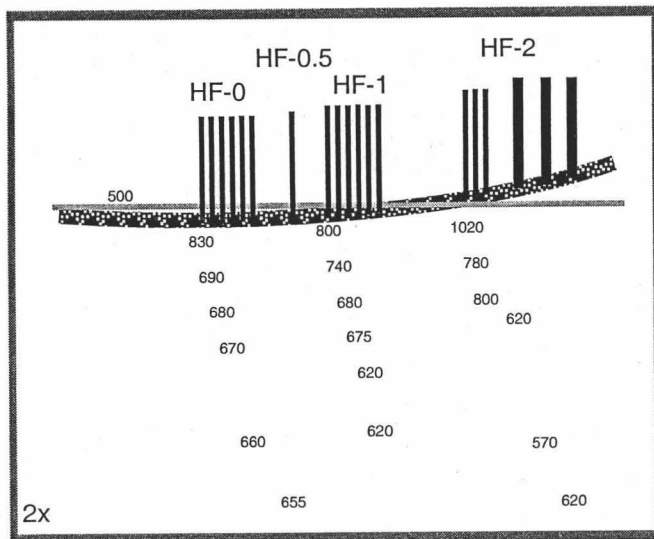
Figure 20. Electrical conductivities in \mu\text{S/cm} at the HF site, 15 September 1996.
