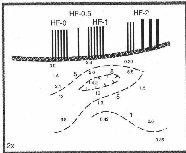
Figure 11. Hydraulic conductivity estimates in m/day at the HF site.
