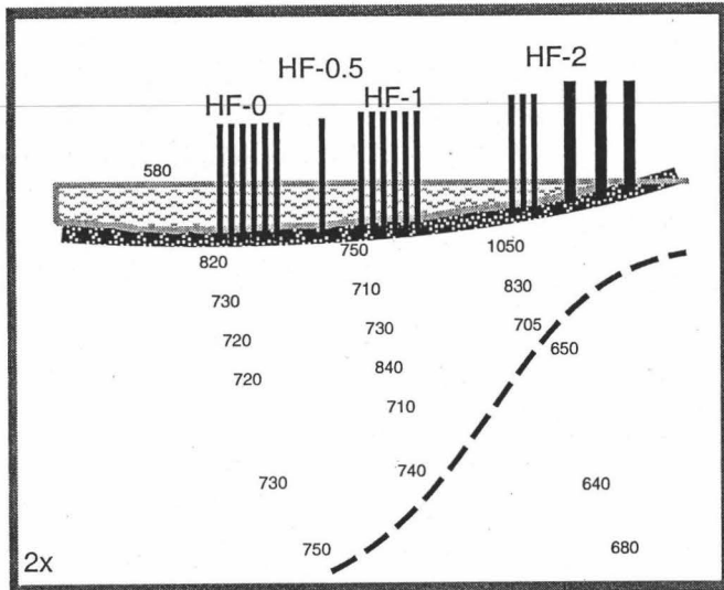
Figure 26. Cross section of the HF site showing a discontinuity in the EC gradient on 8 June 1996. Data are displayed in \mu\text{S/cm} .
