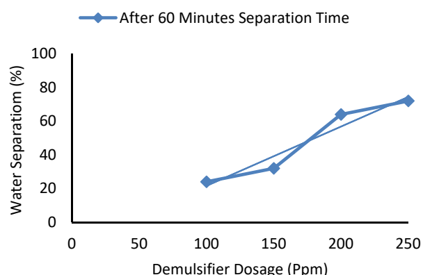
Figure 3. Effect of demulsifier dose variations on the percentage of water separation.
