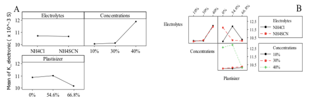
Figure 8. Factorial analysis plot of electrolyte, concentration and plasticizer on electronic conductivity of GPE (A) main factor and (B) interaction between factors
