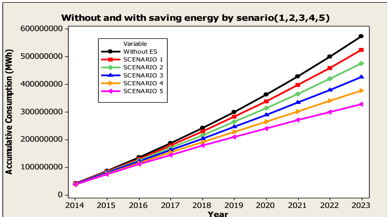
Figure 4: The cumulative energy consumption (MWh) with and without implementing MEES for scenario (1, 2, 3, 4 and 5)
