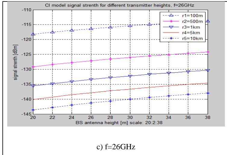
Figure 2: Plot showing received signal strength against BS antenna height for the various distances
