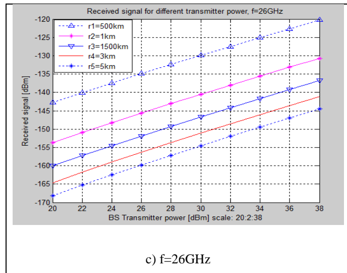
Figure 5: Coverage Prediction Plot showing the impact of transmitted power on coverage area (received signal strength).
