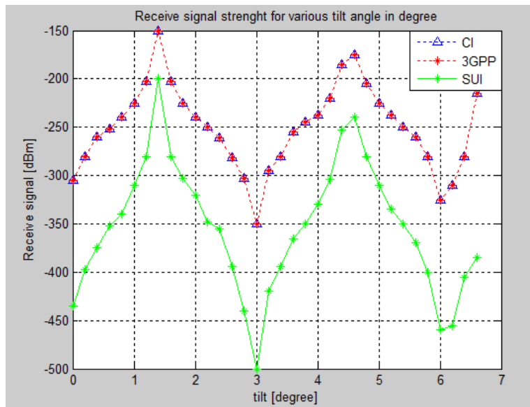
Figure 4: Plot showing the effect of tilt on Received signal level
