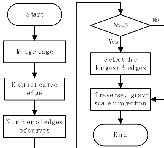
Figure 3: Extract arc
