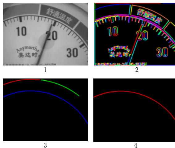
Figure 5: Extraction process
