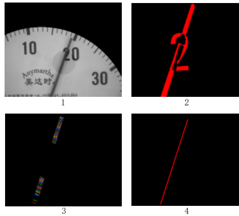
Figure 7: Segment pointer
