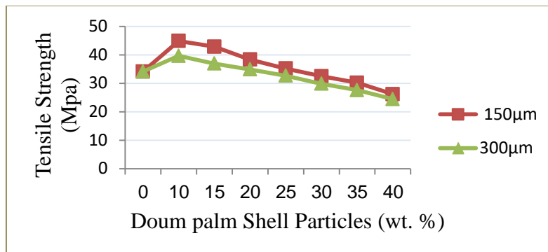
Figure 1: Variation of tensile strength with doum palm shell particle loading.
