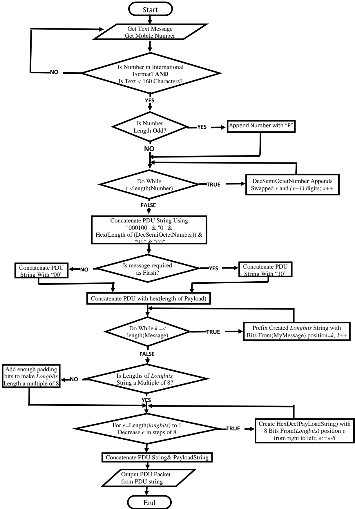
Figure 2: Flow chart for the singular function PDU packing algorithm sequence without an SCA
