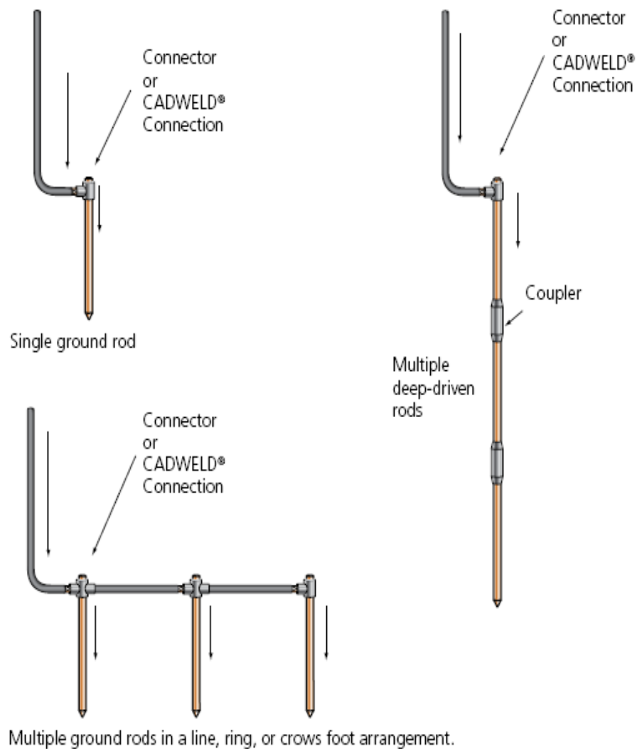
Figure 3: Example vertical electrode arrangements [6]
