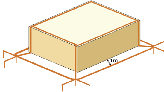
Figure 4: Type B earthing system with additional elements [6]
