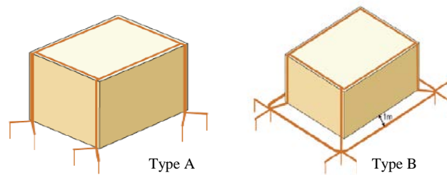
Figure 1: Type A & Type B earthing systems [4]
