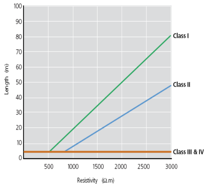
Figure 2: Minimum length of electrodes, l_1 , for Type A & Type B earthing systems [6]
