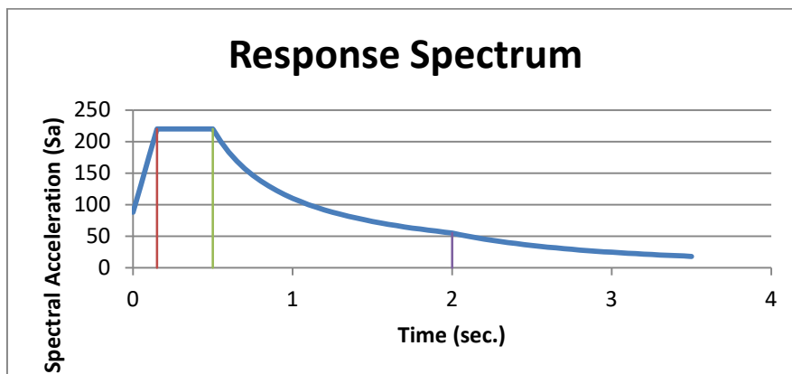
Figure 6: Response Spectrum
