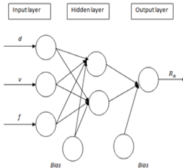
Figure 1: ANN structure
