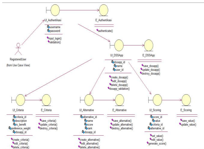
Gambar 2. Class Diagram
