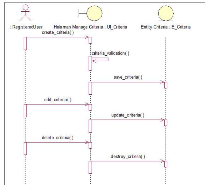
Gambar 5. Sequence Diagram Manage Criteria
