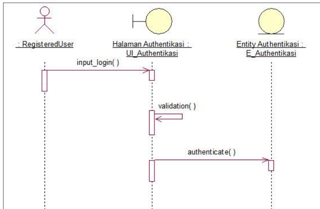
Gambar 3. Sequence Diagram Authentication
