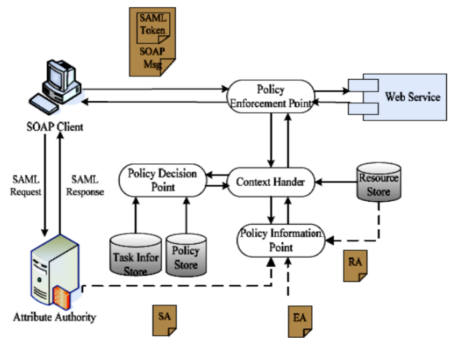
Fig. 6 WABAC Access Control Framework
