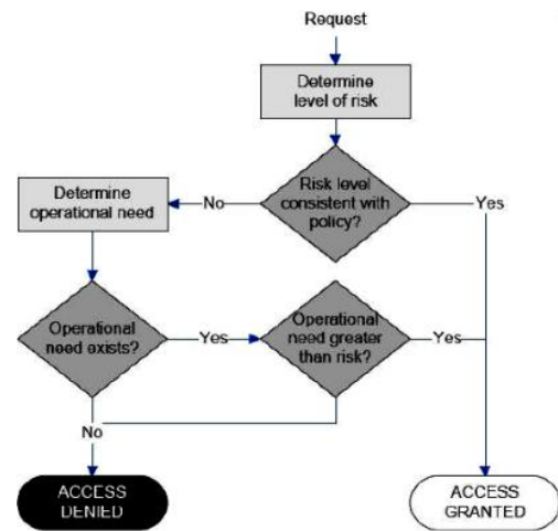
Fig. 5 RAdAC Decision Tree
