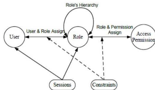
Fig. 3 Role-based access control model
