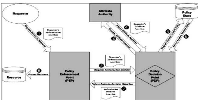
Fig. 4 Use of SAML and XACML in implementing ABAC
