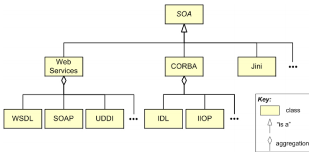
Fig. 1 SOA and SOA Technologies
