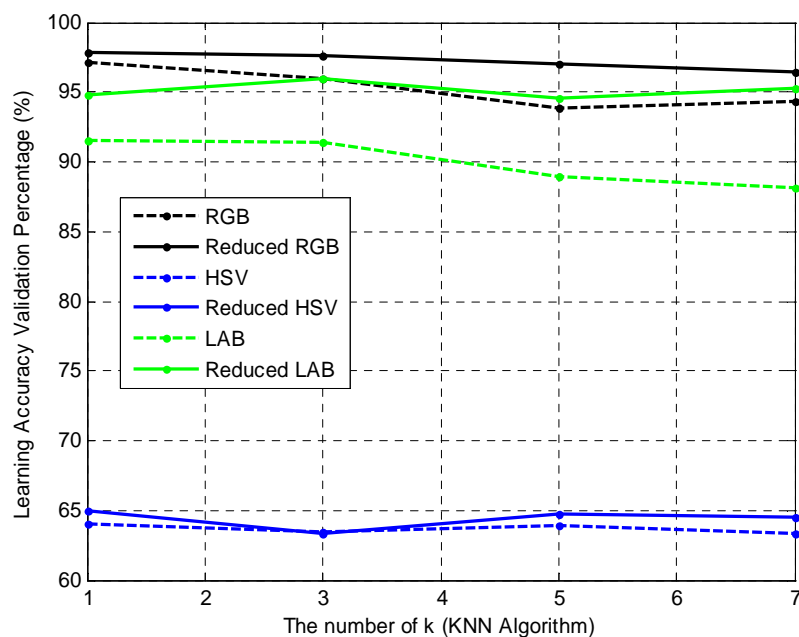
Figure 5. The Accuracy level performance of learning process based on the k value modification using 10 fold cross validation
