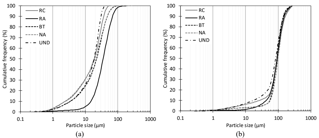
Figure 3. Cumulative particle size distribution of constituents obtained with separate size fractions: (a) < 63 \mu\text{m} , and (b) 63\text{-}125 \mu\text{m} .
