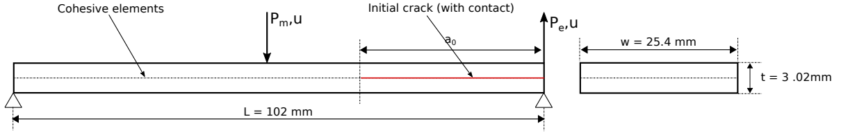
Fig. 6.14 Geometry and loading for mixed-mode bending test
