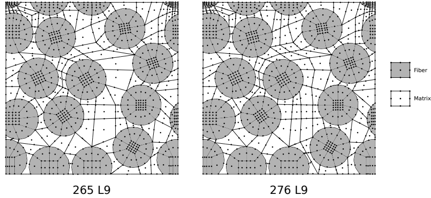
Fig. 4.19 CW discretization of the cross-section of RVE with 13 randomly distributed fibers
