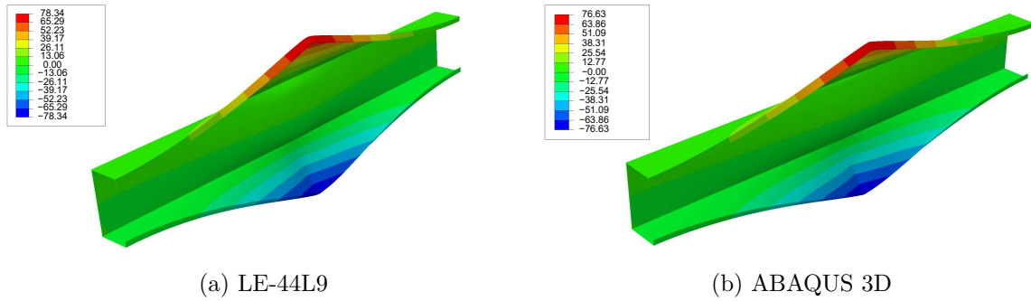
Fig. 3.10 Deformed configuration ( u_z ) at \lambda = 40.98 for fixed-ended lipped channel beam
