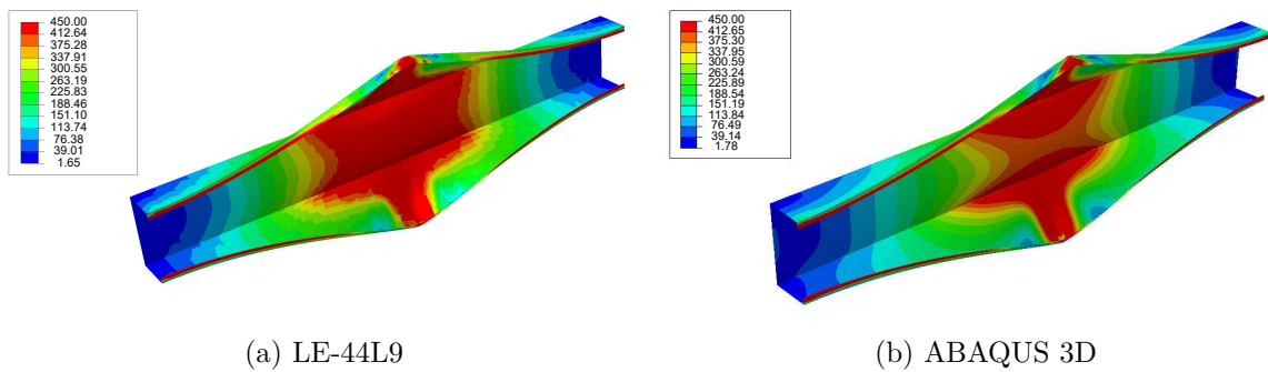
Fig. 3.11 von-Mises stress ( \sigma_{xy} ) distribution at \lambda = 40.98 for fixed-ended lipped channel beam
