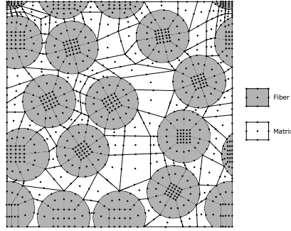
Fig. 4.6 CW discretization of the cross-section of RVE with 13 randomly distributed fibers and a fiber volume fraction of 60%
