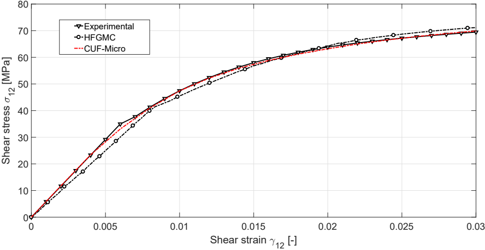
(a) E-Glass/MY750 (Experimental [179] and HFGMC [23])
