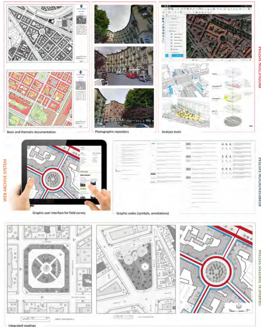
Figure 18. Instrumental components of the integrated system for the survey of urban comfort (SICUR) (edited by Maurizio Marco Bocconcino).
