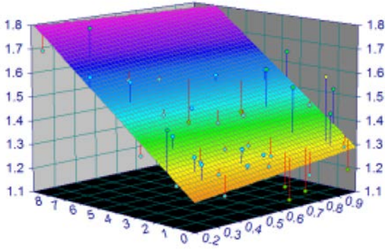
Figure 11. Data interpolation.
