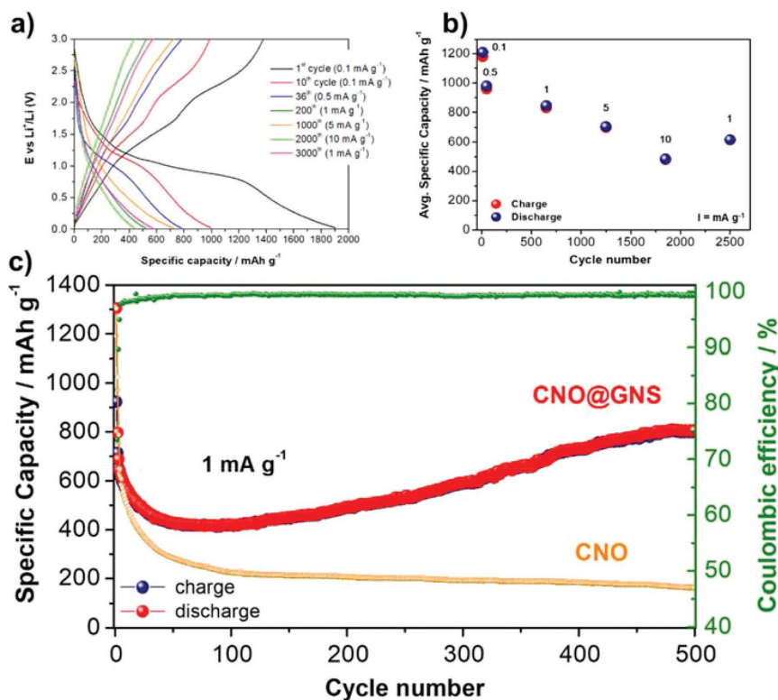
Figure 6. Ambient temperature constant-current (galvanostatic) charge/discharge cycling behavior of the 3D/2D CNO@GNS nanocomposite microspherule electrode: a) potential versus specific capacity profiles and b) rate capability plot at different current densities and cycle number, and c) specific capacity and coulombic efficiency versus cycle number (500 cycles at 1 mA g -1 ) compared to the bare CNO electrode. All current density values ( I ) are given in mA g -1 .
