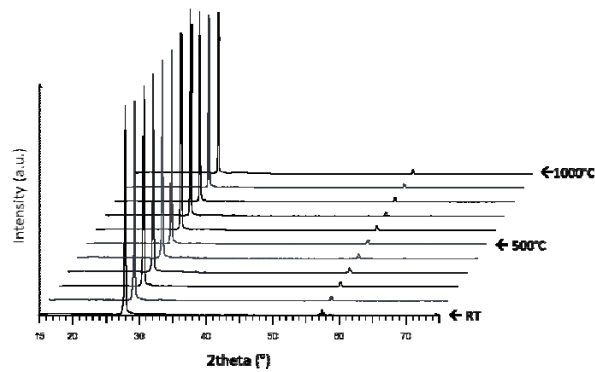
Fig. 4. HT-XRD patterns collected from ambience up to 1000°C by step of 100°C.
