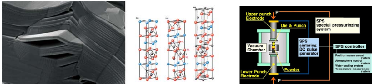
Fig. 1. Micrograph of layered MAX phase [5] and principle of SPS
