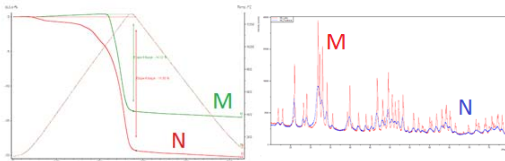
Fig. 4. Dilatometry of both M (green) and N (red) powders (a) and XRD of both powders (b)
