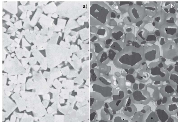
Fig. 1. Grain structure of a) WC-18Co cemented carbide and b) TiCN5WC10Co cermet. The cobalt is bright in the cermet and darker in the WC-Co. In the cermet, the typical core-rim structure can be observed
