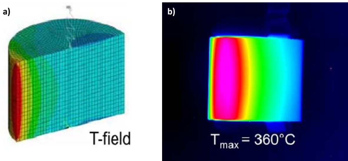
Fig. 5. Temperature distribution in the axial mid plane of a varistor with local inhomogeneities in service: (a) simulation and (b) measurement.
