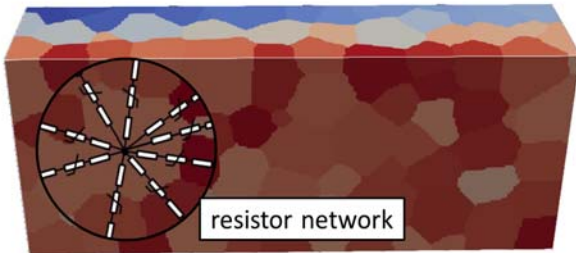
Fig. 7. 3D model of the ZnO microstructure as a basis for a resistor network.
