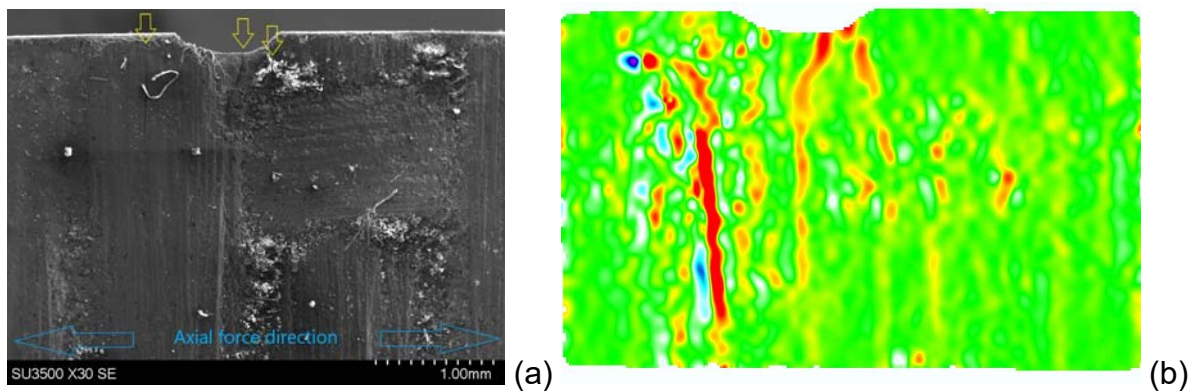
Fig. 3. Notched SiC z /SiC tensile test result (a) SEM Image (b) DIC Image 50 Newtons from failure.
