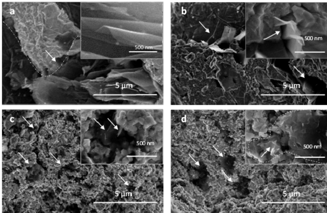
Fig.1. SEM micrograph showing the morphology of the ceramic grains and arrowed GBNs in composites with 10 vol% GNP processed with: (a) ultrasound probe (u.p.), (b) u.p. and wet milling, (c) dry milling, (d) u.p. and dry milling. The inserts show zoomed areas.
