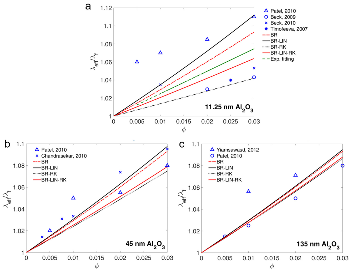
Fig. 5. Comparison between modeling (lines) and experimental (dots) values of thermal conductivity enhancement for nanofluids made of water and alumina nanoparticles with different diameters: (a) 11.25 nm; (b) 45 nm; (c) 135 nm. Models are defined according to Table 1; experimental data are extracted from the references in Table 2. Note that the dashed green line in panel (a) is a linear fitting of the reported experimental results.
