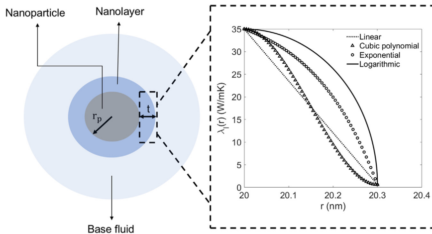
Fig. 1. Thermal conductivity profile in the water nanolayer in proximity of an alumina nanoparticle ( \lambda_f = 0.60 W/m K, \lambda_p = 35 W/m K [29], r_p = 20 nm and t = 0.30 nm [30,26]). The thermal conductivity profiles in the nanolayer predicted by Eqs. (6)–(9) are compared.
