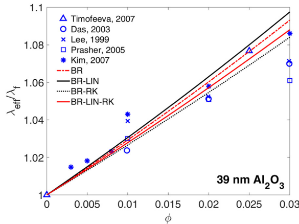
Fig. 3. Comparison between modeling (lines) and experimental (dots) values of normalized effective thermal conductivity of nanofluids made of water and alumina nanoparticles (39 nm diameter). The reported models are defined according to Table 1; whereas, experimental data are extracted from the references in Table 2.
