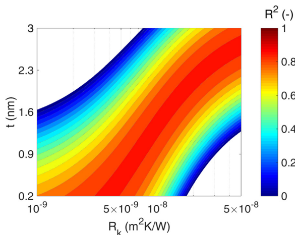
Fig. 4. Coefficient of determination ( R^2 ) of BR-LIN-RK model fitting to the experimental results reported in Fig. 3, with different values of Kapitza resistance ( R_k ) and nanolayer thickness ( t ) at the alumina-water interface. For the sake of clarity, combinations of R_k and t leading to R^2 < 0 are colored in white.
