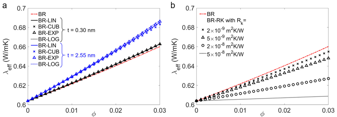
Fig. 2. Sensitivity analysis of the effective thermal conductivity with respect to (a) nanolayer thermal conductivity profile and (b) Kapitza resistance. The reported models are defined according to Table 1 and refer to alumina-water nanofluid.
