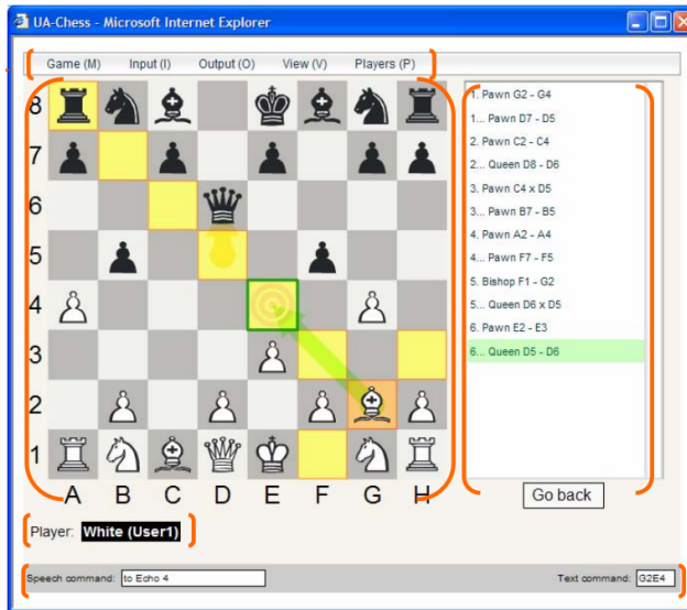
Fig. 3. UA-Chess main user interface
