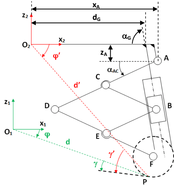
Fig.19 – Schematic representation of the proposed mechanism
