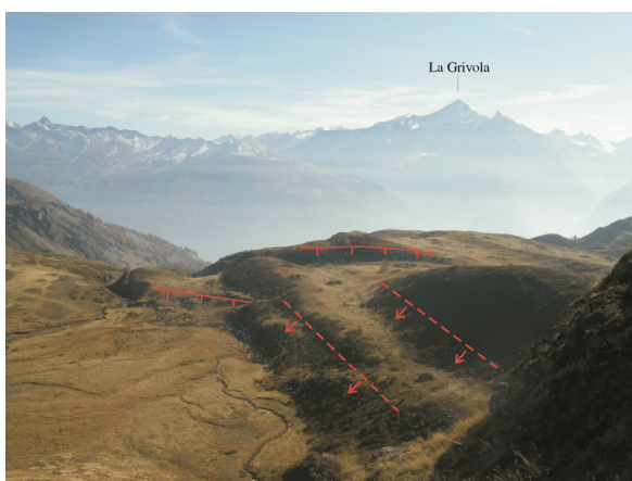
Fig. 11 - Wide horizontal surface that corresponds to the Plan di Modzon filled lake, bounded by minor scarps (shaped lines) and counterscarps (continuous lines) that form a barrier to the flow of watercourse.
