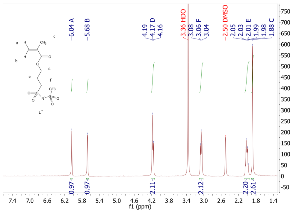
Figura 4.3 ^1\text{H} NMR of lithium 1-[3-(methacryloyloxy)propylsulfonyl]-1-(trifluoromethylsulfonyl)imide recorded in \text{DMSO-d}_6
