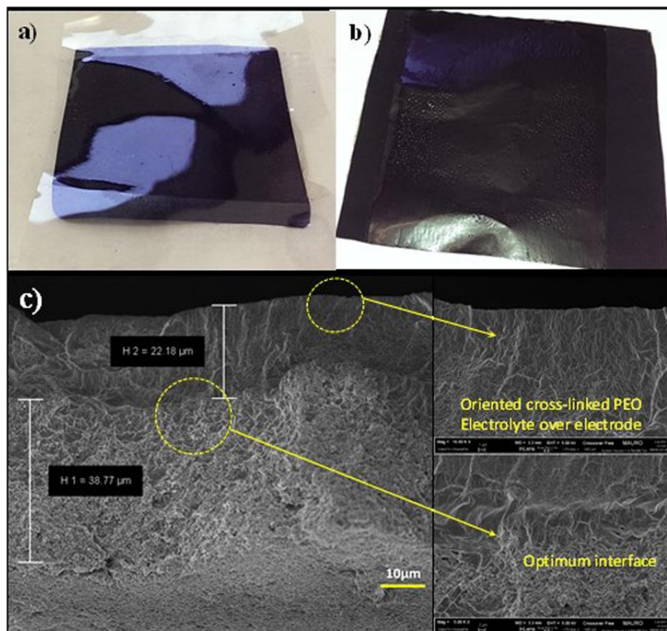
Figure 3.13 (a) Photograph of bare \text{TiO}_2 based electrode and electrolyte before UV curing. (b) Freshly prepared self-supporting multiphase electrode/electrolyte composite obtained by direct hot-pressing and in situ photopolymerisation of the polymer electrolyte over the \text{TiO}_2 -electrode film supported over copper foil. (c) Cross-sectional FESEM images showing the optimum interface achieved after UV curing.
