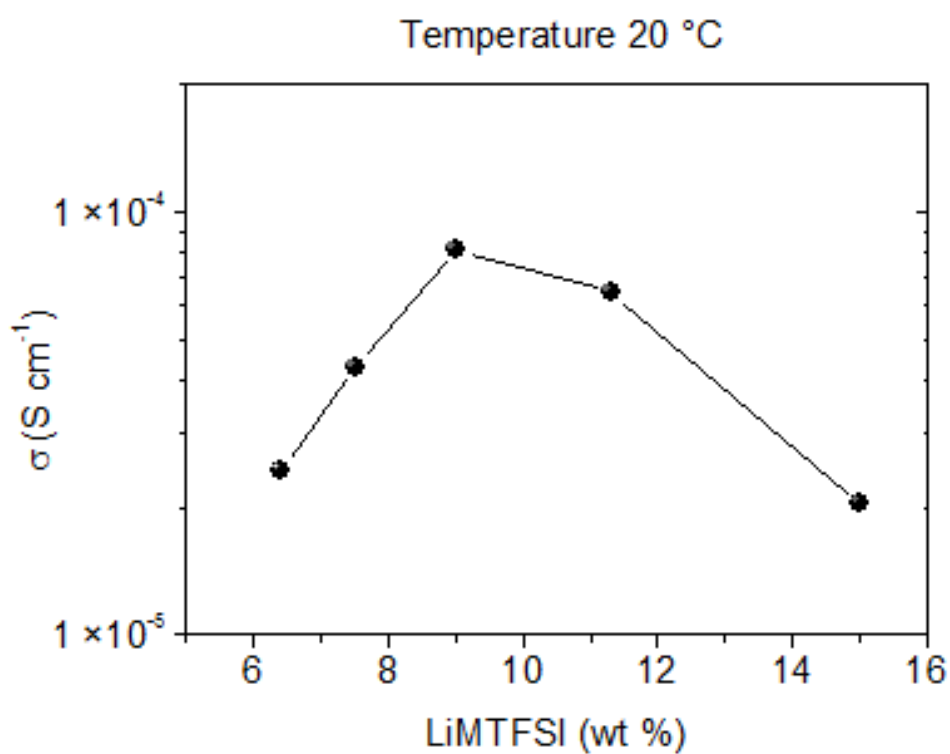
Figure 5.4 Dependence of ionic conductivity on \text{Li}^+ concentration under isothermal conditions (20 °C).
