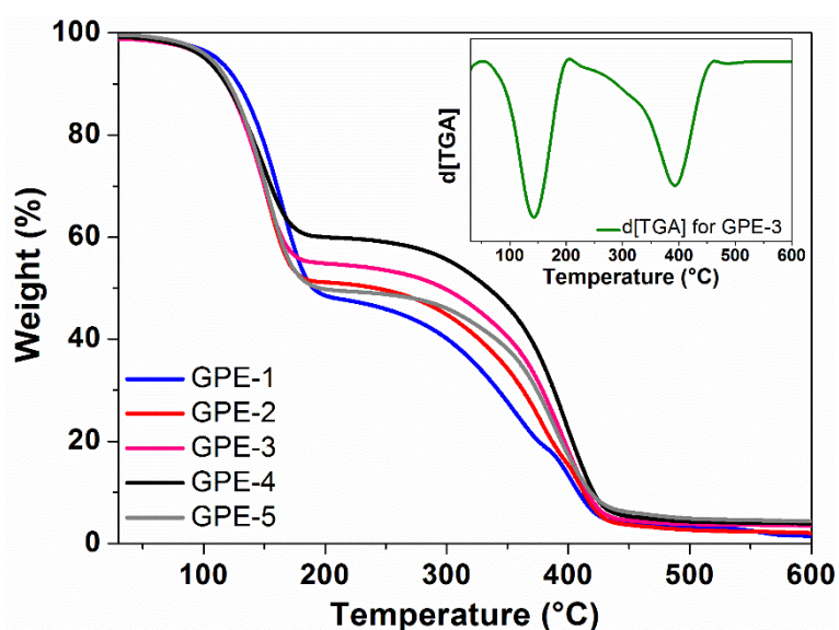
Figure 5.2 TGA traces, measured under N_2 from 30 to 600 °C, of the GPE samples under study, the differential curve of sample GPE-3 is shown in the inset.
