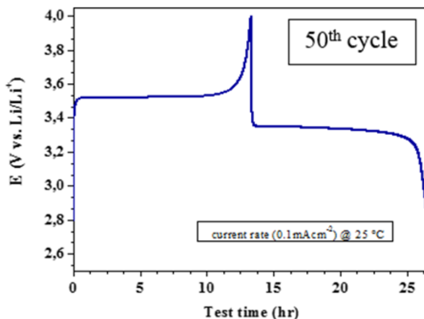
Figure 3.16 Charge/discharge curve of a lithium test cell assembled with a configuration of Li/PTL-1/LiFePO 4 . The test was performed at 25 °C at current densities of 0.1 mA cm -2 .
