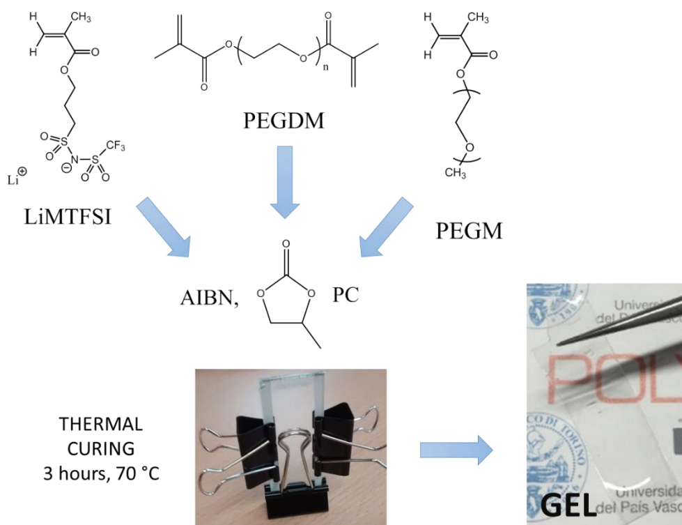
Scheme 5.1 Sketched preparation procedure of single-ion GPEs, along with the structure of the reagents and the aspect of the final polymer electrolyte.
