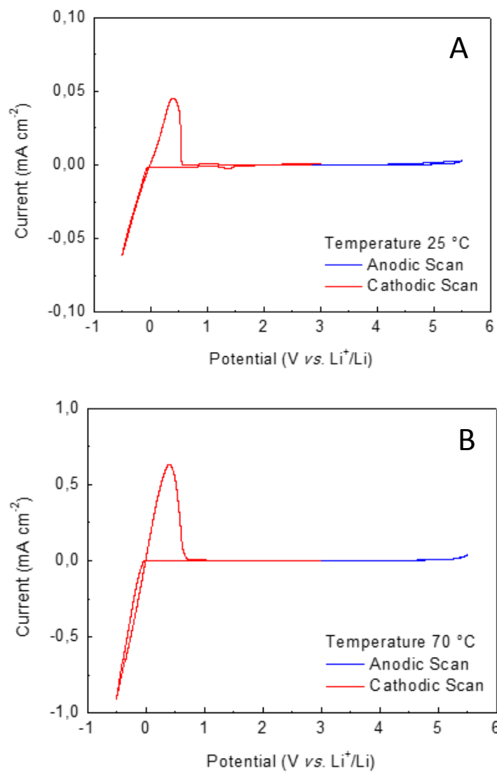
FIGURE 5.6 Electrochemical window of GPE-3 obtained by CV in the -0.5 – 5.5 V vs. Li + /Li interval at a scan rate of 0.2 mv s -1 and different temperatures: (a) 25 and (b) 70 °C.
