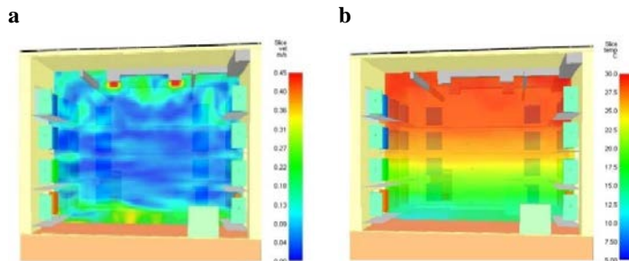
Fig. 3. (a) Computational thermal-fluid-dynamic simulation of the indoor air velocity field at the mock-up; (b) computational thermal-fluid-dynamic simulation of the indoor air temperature field at the mock-up
