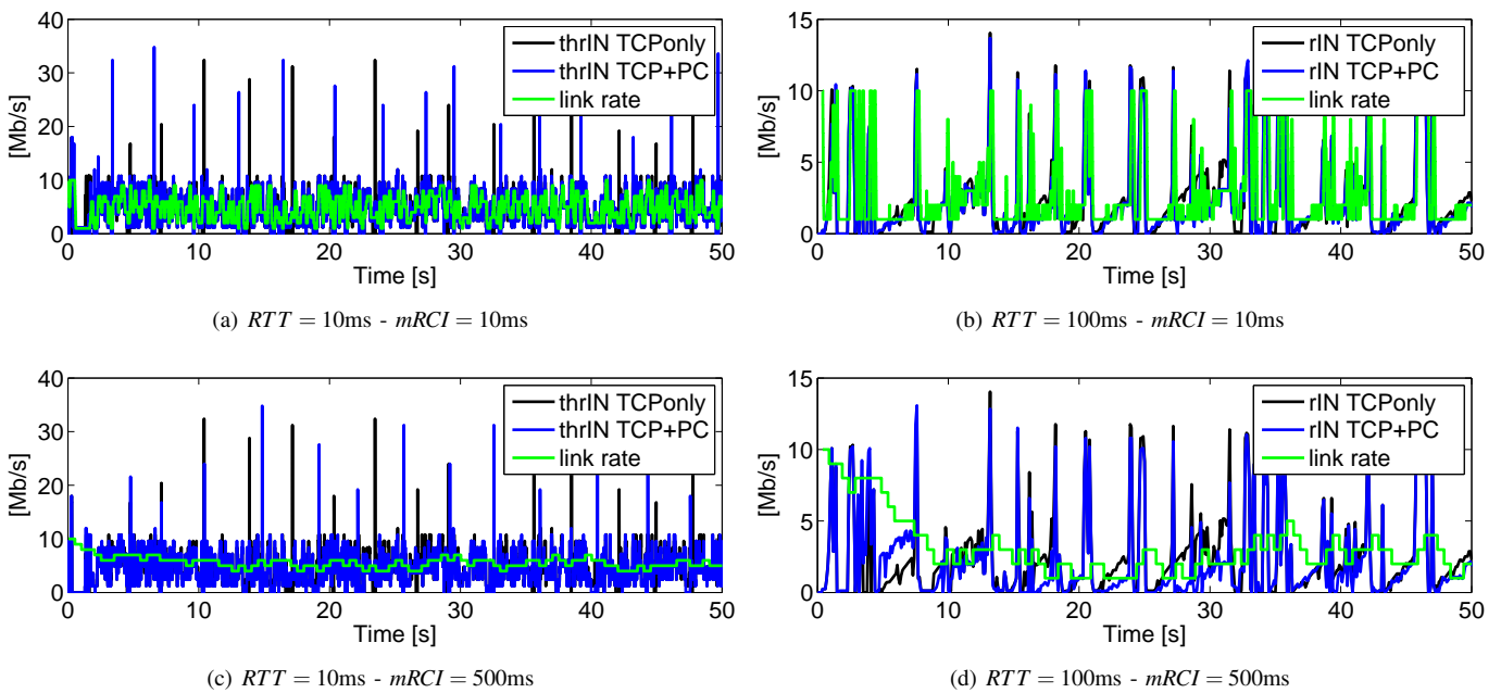
Fig. 7. Bottleneck ( BN = 50\text{ms} ) - Background Traffic ( bON = 100\text{ms} ): Comparison between the temporal evolution of the service rate chosen by the capacity scaling algorithm and the temporal evolution of the arrival rate at node N1 in the TCP+PC and TCPOnly cases
