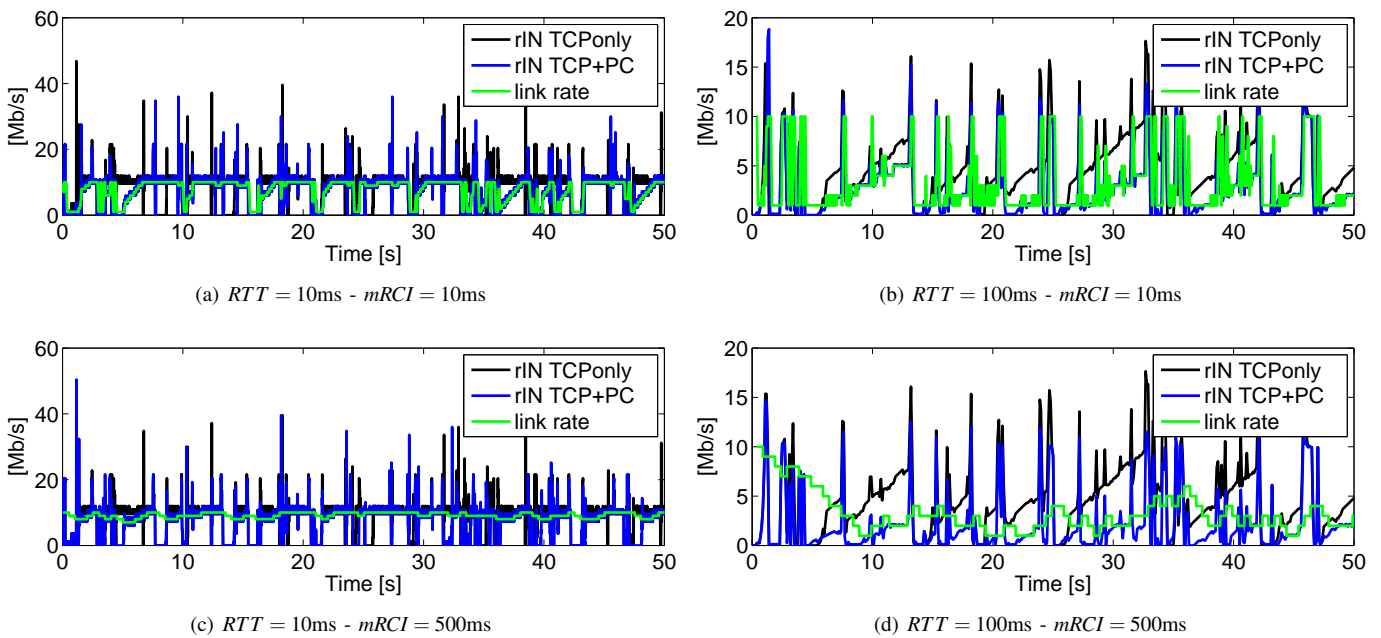
Fig. 5. Background Traffic ( bON = 100ms ): Comparison between the temporal evolution of the service rate chosen by the capacity scaling algorithm and the temporal evolution of the arrival rate at node N1 in the TCP+PC and TCPOnly cases
