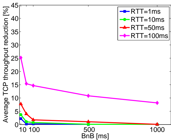
(b) Average TCP throughput reduction in the TCP+PC case with respect to the TCPonly case
