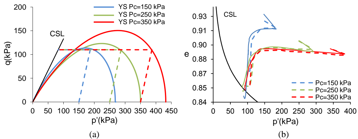
Figure 6. Effect of consolidation stress on sand experimental behavior (dashed line) and model prediction (solid line) in the CSL loading: (a) Stress paths (b) Void ratio changes.
