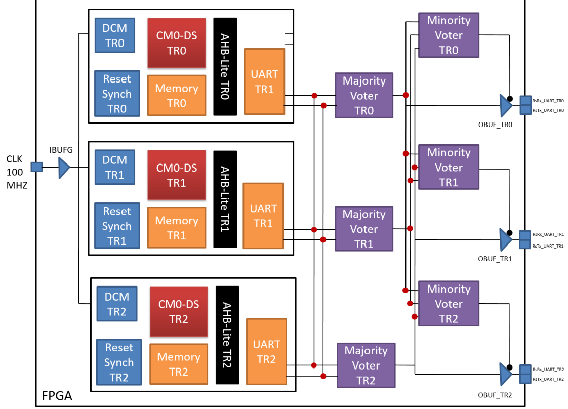
Figure 6.9: Architecture of ARM SoC with XTMR applied on Virtex-5 FPGA
