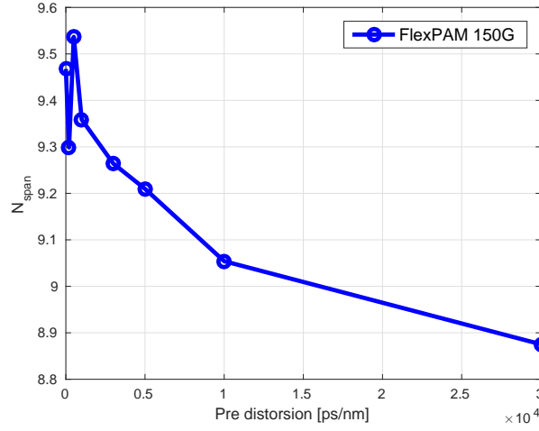
Figure 6.23. The maximum reach of FlexPAM 150G in different pre distortion. Noted that the target BER is 10^{-3} in this case.
