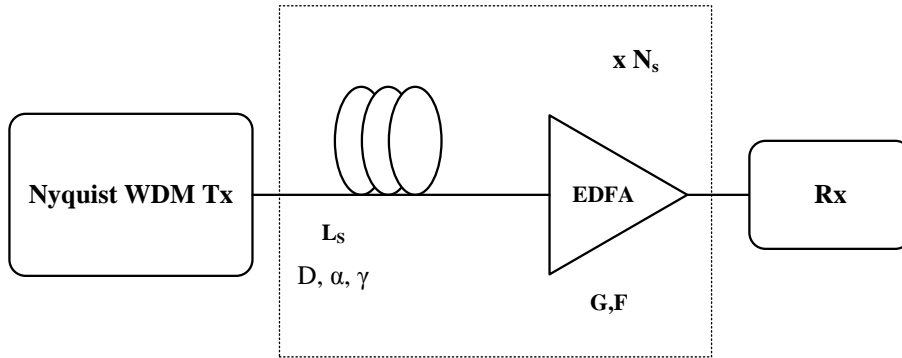
Figure 5.8. 13 Nyquist WDM channels with 50 GHz channel spacing are combined together and transmitted through the coherent link. The SSMF is employed. The fiber span lose is fully recovered by the amplifier.
