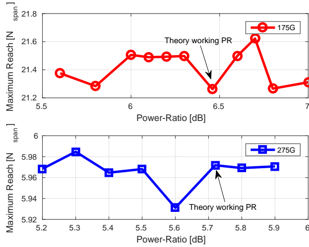
Figure 6.20. Power-ratio tuning in Flex-PAM 175G and 275G, whose format-ratio \kappa = 0.25 . System performance did not benefit from the power-ratio tuning.
