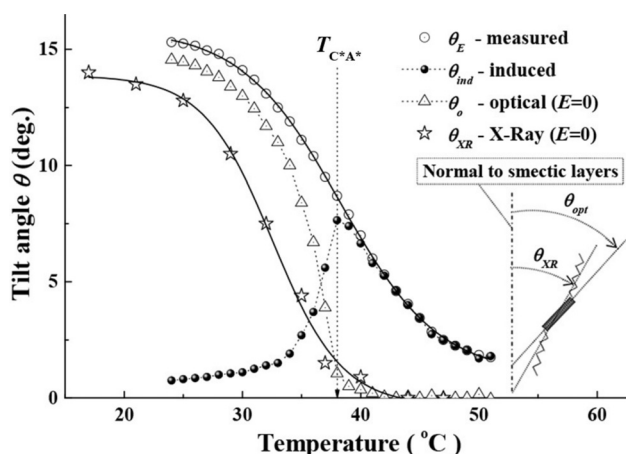
FIG. 3. Dependencies of NFLC-1 tilt angle on temperature. \theta_E , \theta_{ind} refer to the applied field E_1 = 6.67 V/ \mu m. The inset shows the zig-zag model 14 representation.
