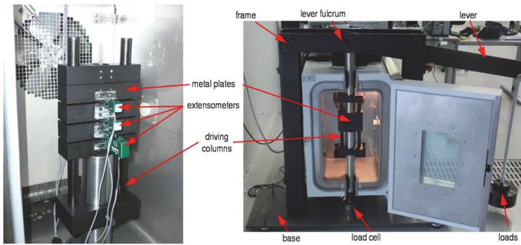
Figure 3. Testing machine.
