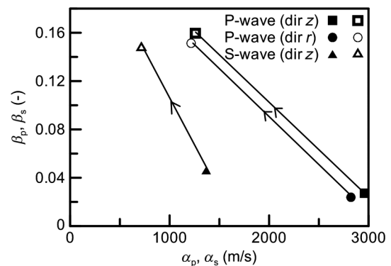
Figure 4. Case history 1: effect of sample destructuration on \alpha_i and \beta_i .
