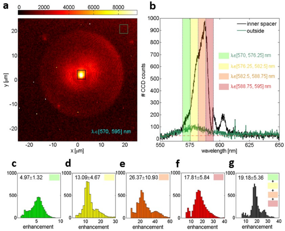
Figure 5.10: (a) False-color image of the circular grating as obtained by means of the BFP scanning system. Intensity values are integrated over a spectral range from \lambda = 570 \text{ nm} to \lambda = 595 \text{ nm} . (b) Fluorescence spectra corresponding to the grating inner spacer and outside the grating. Coloured bars indicate spectral intervals used for further analysis. (c-g) statistical distributions of the enhancement factor calculated over the corresponding spectral ranges. Average and standard deviation are indicated for each spectral range.
