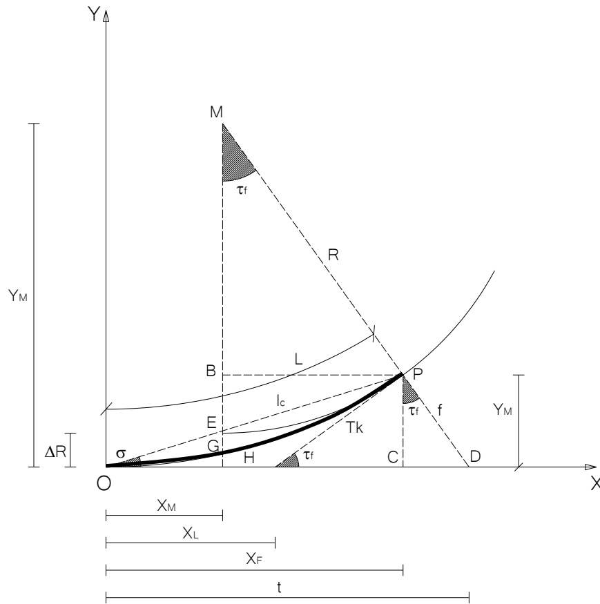
Figure 3.3 - Clothoid general scheme
