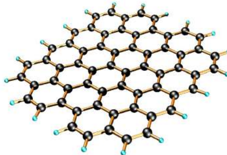
Figure 1.1. Honeycomb lattice structure of an idealized SLG. It can be seen as the starting base of all the allotropes of carbon.
