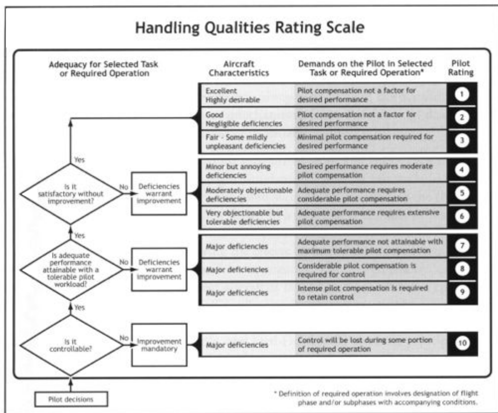
Figure 9.6: Cooper-Harper rating scale [3]
