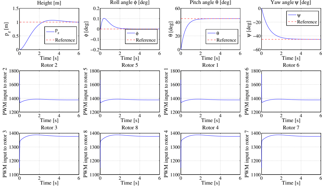
Figure 9.2: Nonlinear dynamics of a LQ regulated aggressive maneuver; the rotors position in the figure recalls the physical rotors position in the multirotor
