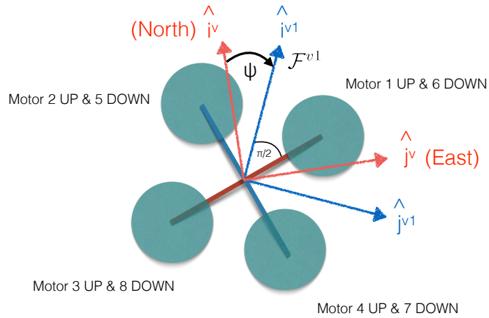
Figure 2.6: The vehicle-1 frame. If the roll and pitch angles are zero, then the x -axis points out the nose of the airframe, the y -axis points out to the right and the z -axis points into the earth
