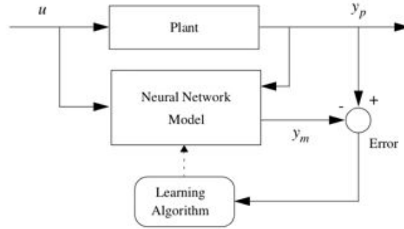
Figure 10.14: Plant identification
