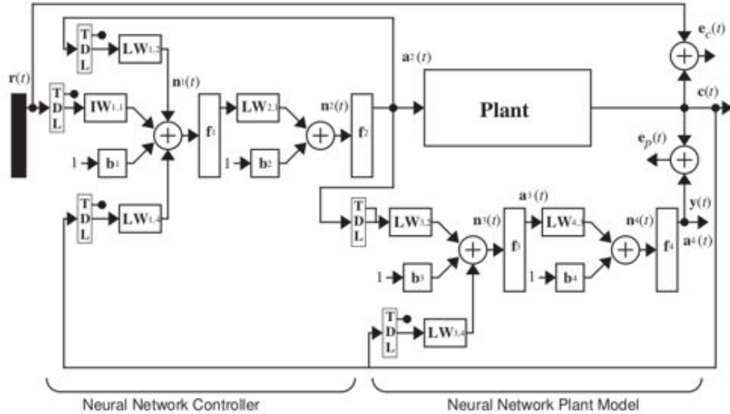
Figure 10.17: Detailed model reference control structure
