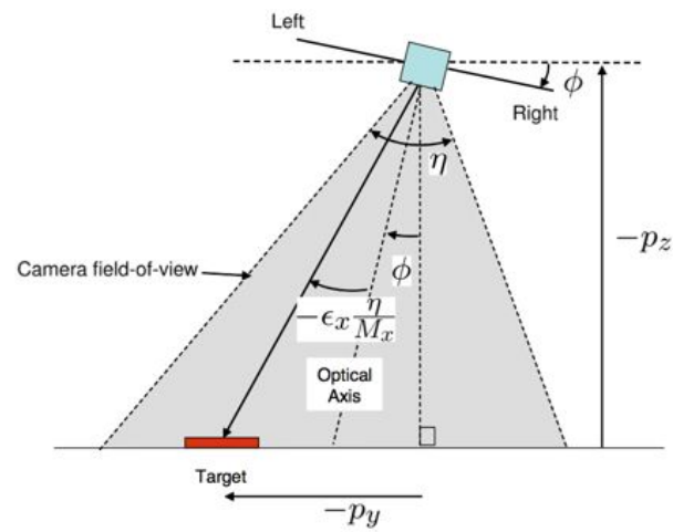
Figure 6.2: Geometry introduced by the vision system. The height above ground is given by -p_z , the lateral position error is p_y , the roll angle is \phi , the field-of-view of the camera is \eta , the lateral pixel location of the target in the image is \epsilon_x and the total number of pixels along the lateral axis of the camera is M_x .
