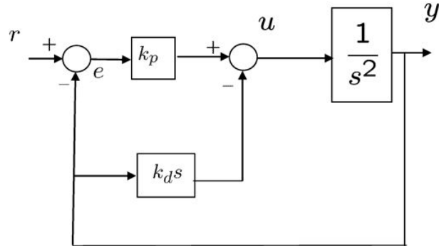
Figure 8.3: Standard PD loop
