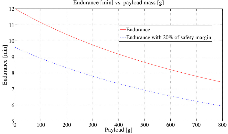
Figure 4.4: Multirotor endurance as a function of the payload mass
