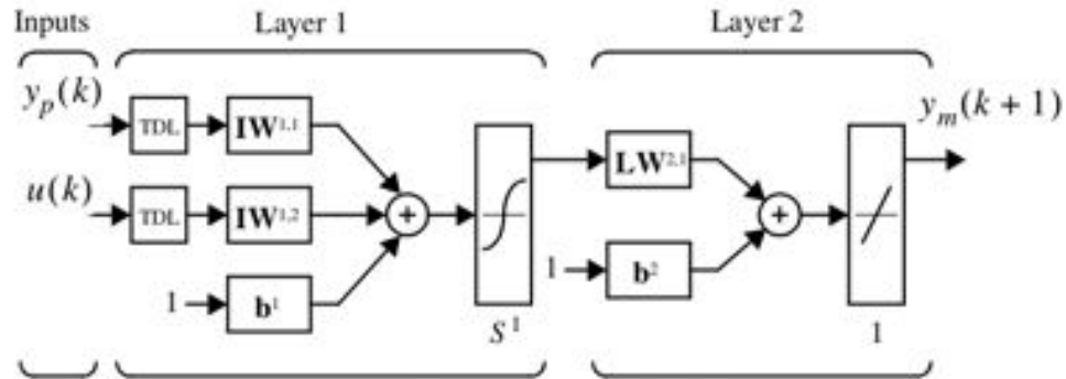
Figure 10.15: Neural network plant model
