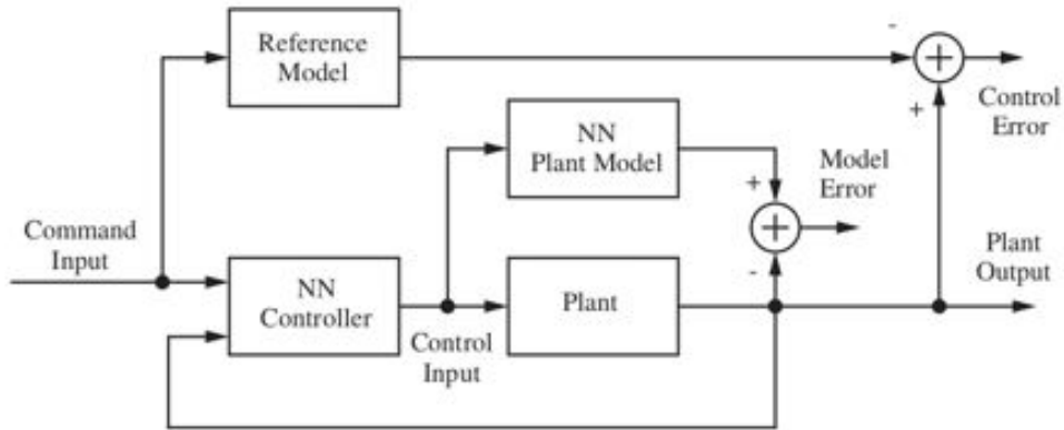
Figure 10.16: Model reference control architecture
