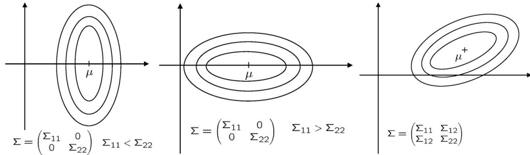
Figure 7.2: Level curves for the probability density function of a 2D Gaussian random variable
