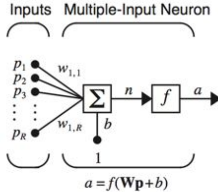
Figure 10.4: Multiple-input neuron
