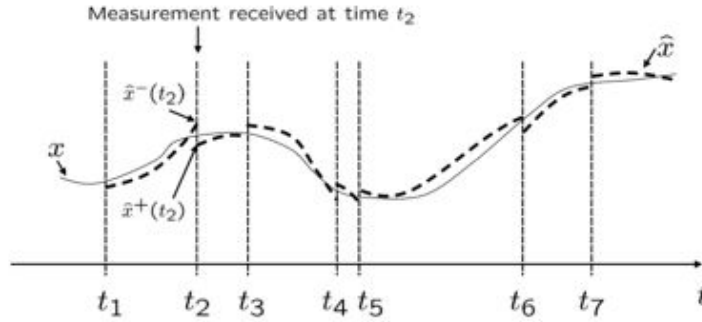
Figure 7.1: Observation process
