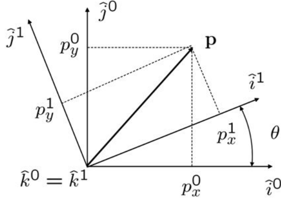
Figure 2.1: Rotation in 2D
