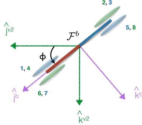
Figure 2.8: The body frame. The x -axis points out the nose of the airframe, the y -axis points out the right and the z -axis points out the belly
