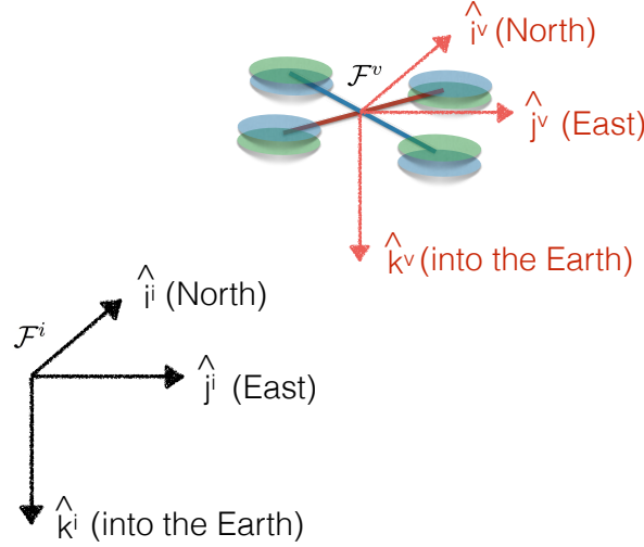
Figure 2.5: The vehicle coordinate frame. The x -axis points North, the y -axis points East and the z -axis points into the earth
