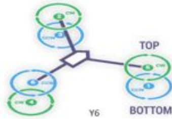
Figure 1.18: Hexarotor Y design configuration
