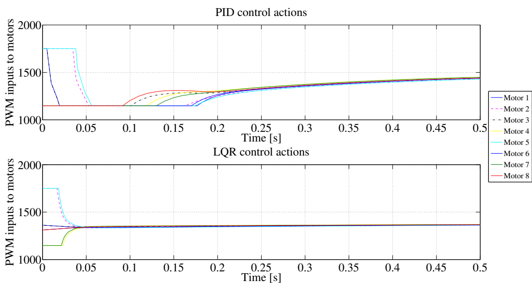
Figure 9.4: Control actions: PID vs. LQR
