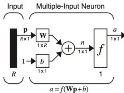
Figure 10.5: Neuron with R inputs, matrix notation
