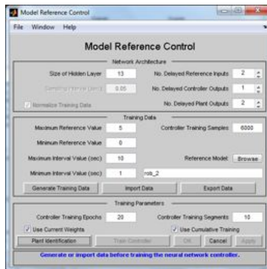
Figure 10.19: Matlab graphical user interface for the neural network controller identification and training
