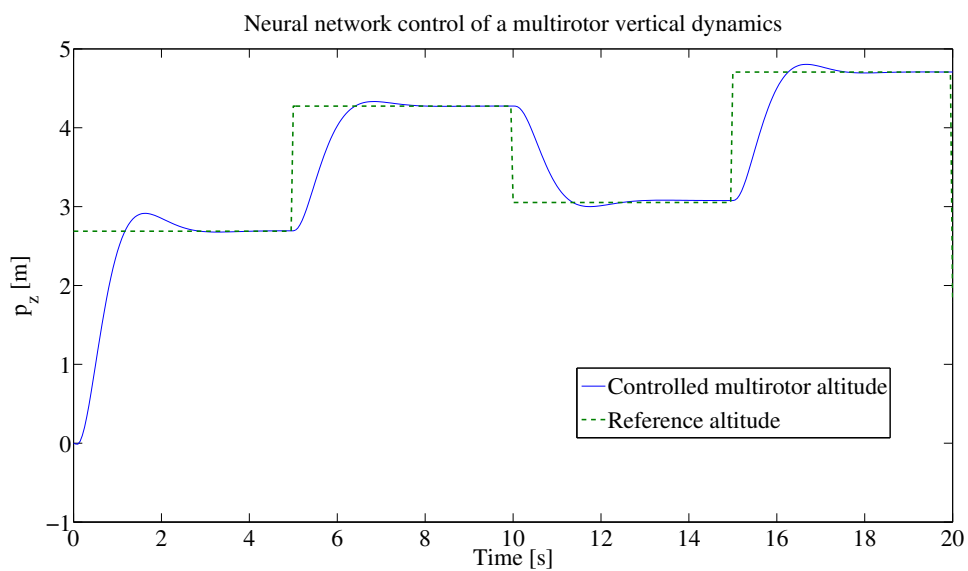
Figure 10.20: Neural network controlled vertical position
