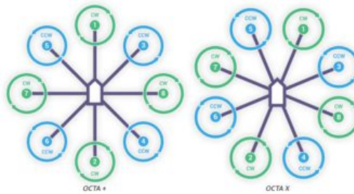
Figure 1.16: Octorotor + and X flight configurations
