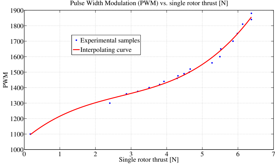
Figure 5.1: PWM_i(F_i) relation
