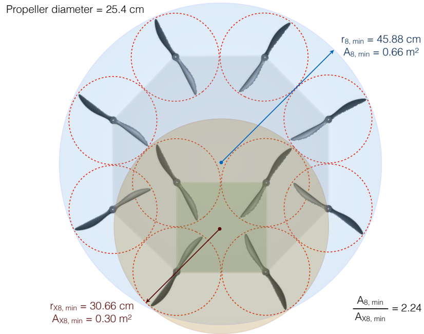
Figure 4.6: Comparison between the classical and X8 octorotor minimum size
