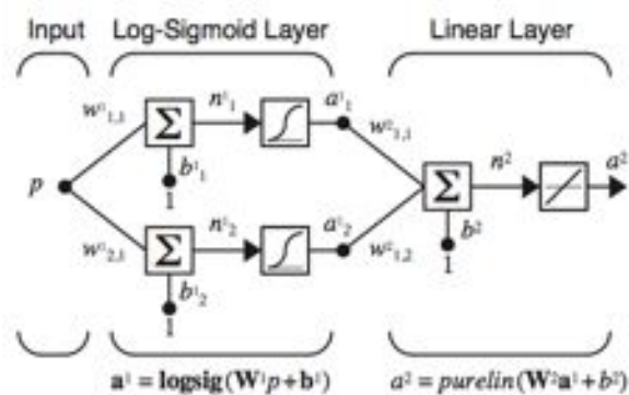
Figure 10.9: Example function approximation network
