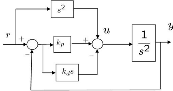
Figure 8.4: Feedforward term is added to a standard PD loop
