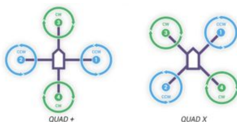
Figure 1.14: Quadrotor + and X flight configurations
