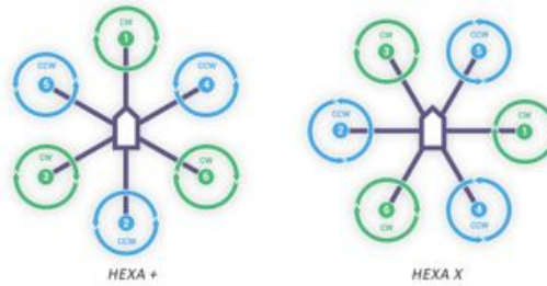
Figure 1.15: Hexarotor + and X flight configurations
