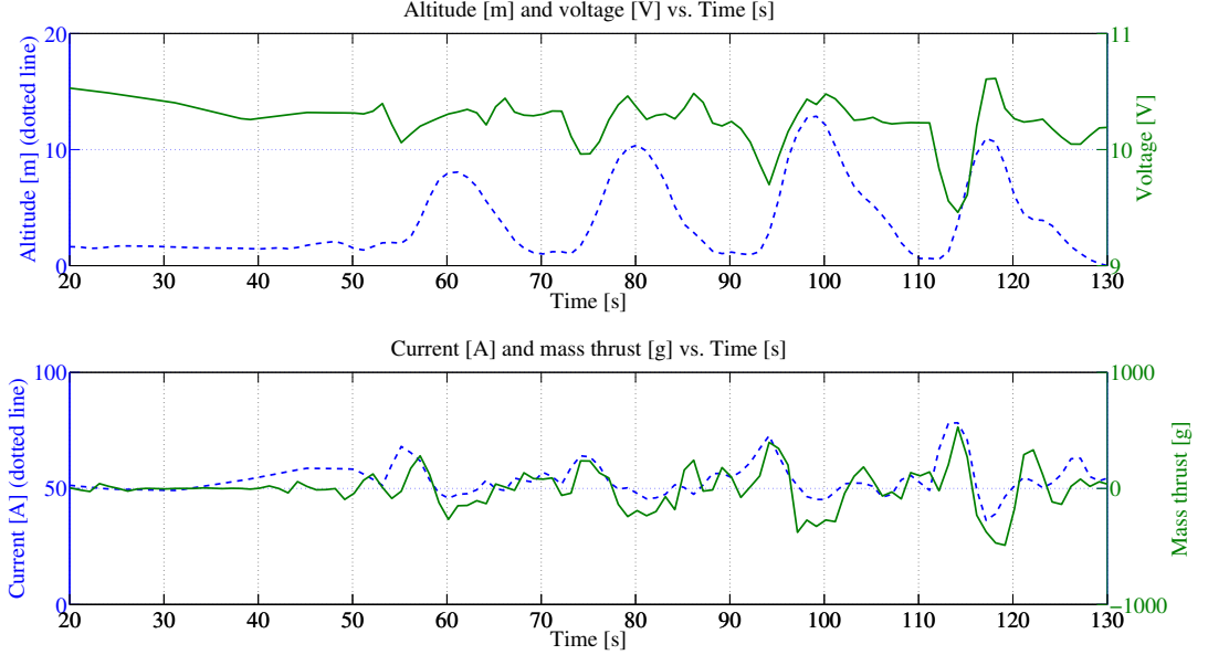
Figure 4.3: Parameters measured during the sequence of vertical accelerations
