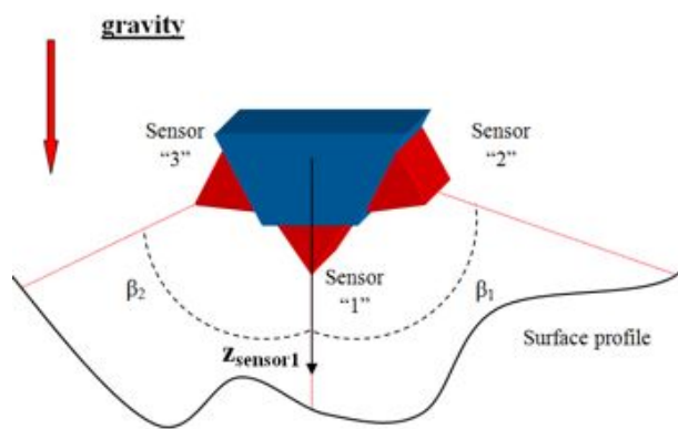
Figure 10.25: A three sensors setup
