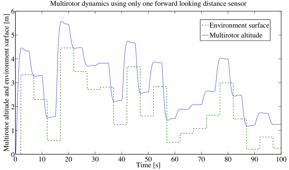
Figure 10.24: Multirotor dynamics using only one forward looking distance sensor
