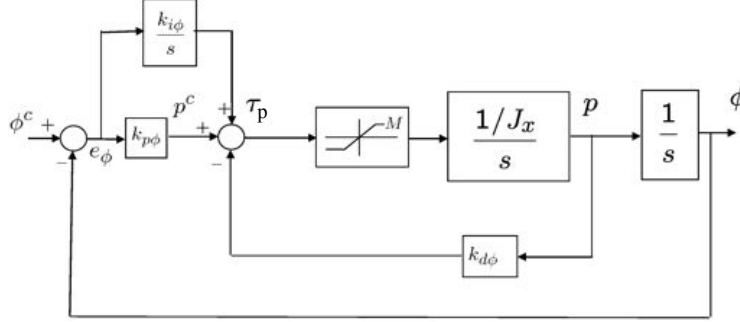
Figure 8.2: A block diagram of the roll attitude hold loop
