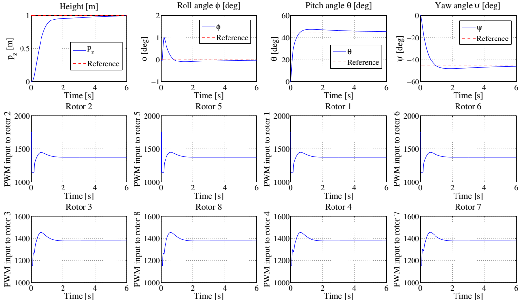
Figure 9.1: Nonlinear dynamics of a PID regulated aggressive maneuver; the rotors position in the figure recalls the physical rotors position in the multirotor
