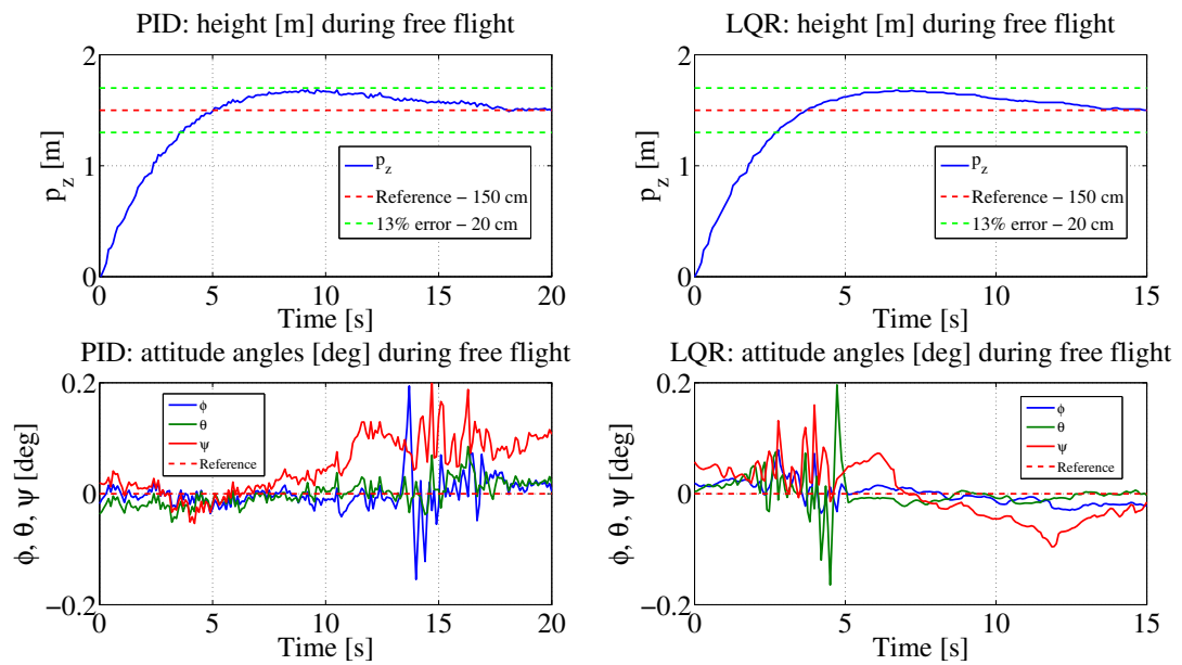
Figure 9.10: PID and LQR controlled height and attitude angles during free flight
