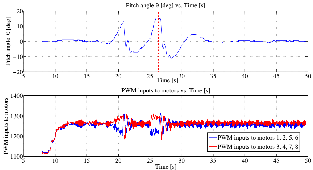
Figure 9.8: Experimental PID controlled pitch output and relevant motors inputs
