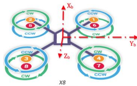
Figure 1.19: Octorotor X flight and design configuration
