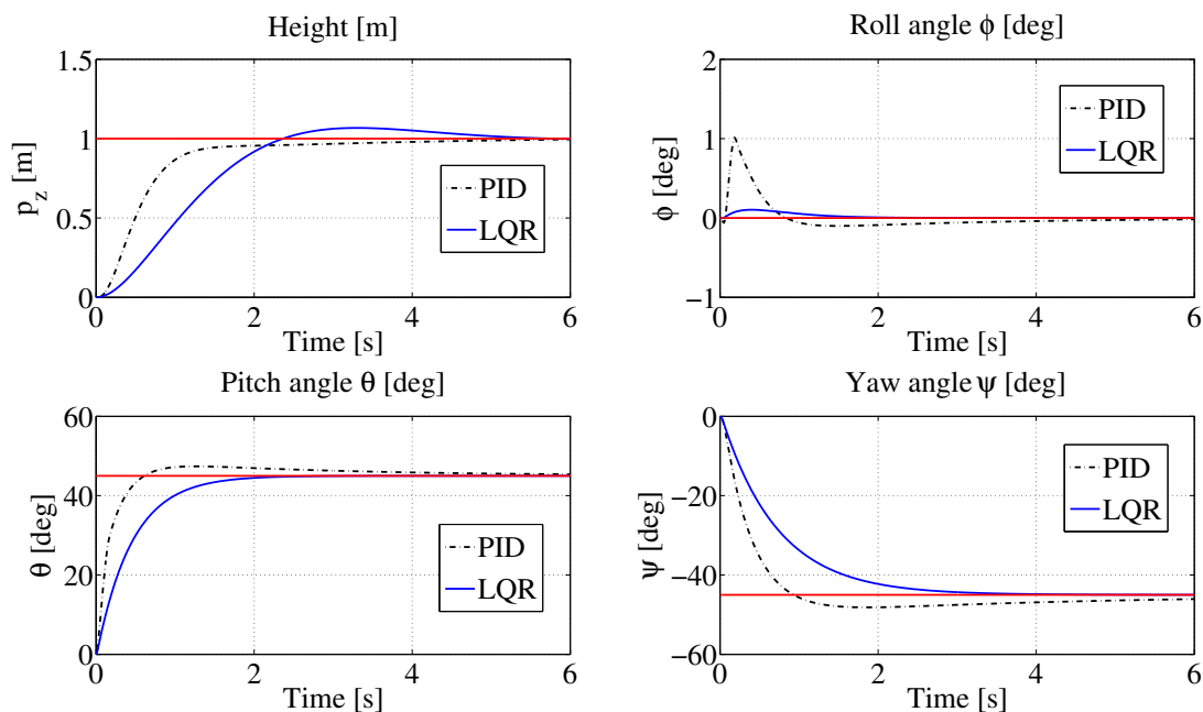
Figure 9.3: Height ( p_z ), roll ( \phi ), pitch ( \theta ) and yaw ( \psi ) angles regulation performance: PID vs. LQR
