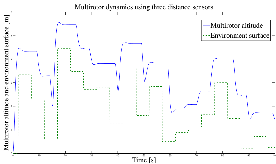
Figure 10.26: Multirotor dynamics using three distance sensors
