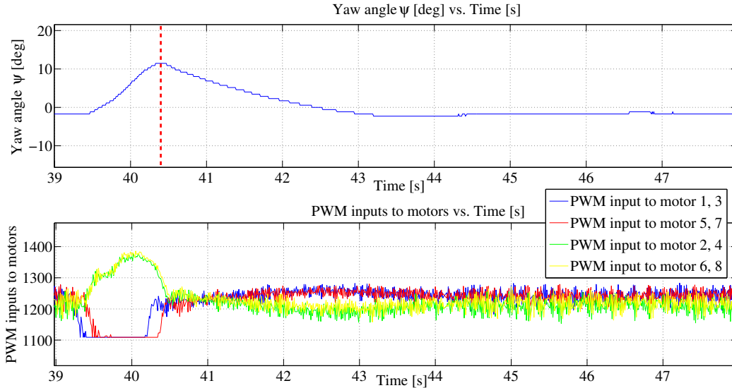
Figure 9.9: Experimental LQ regulated yaw output and relevant motors inputs
