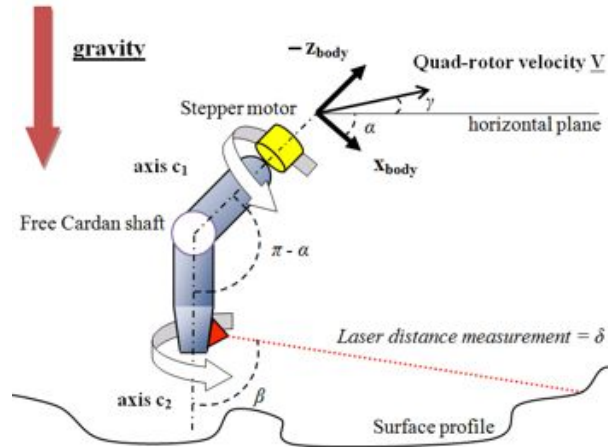
Figure 10.22: Distance sensor embodiment
