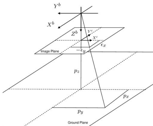
Figure 6.1: Camera model for the multirotor
