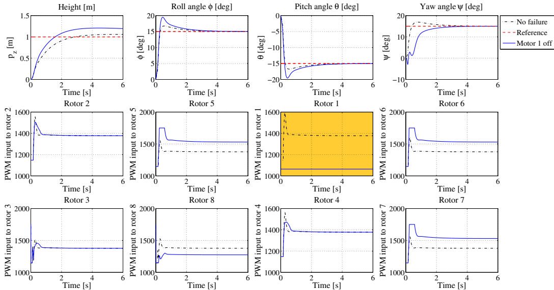
Figure 9.5: PID control simulation in case of motor “1” failure
