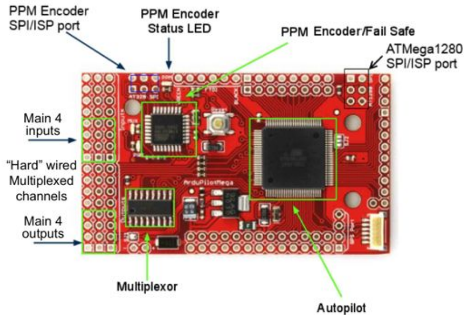
Figure 4.1: The Ardupilot Mega board
