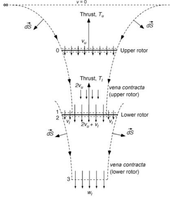
Figure 4.5: Flow model for a coaxial rotor analysis where the lower rotor is considered to operate in the fully developed slipstream of the upper rotor [2]
