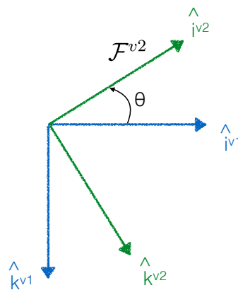
Figure 2.7: The vehicle-2 frame. If the roll angle is zero, then the x axis points out the nose of the airframe, the y -axis points out the right and the z axis points out the belly
