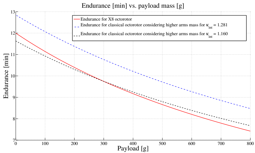
Figure 4.7: Comparison between the classical and X8 octorotor endurance
