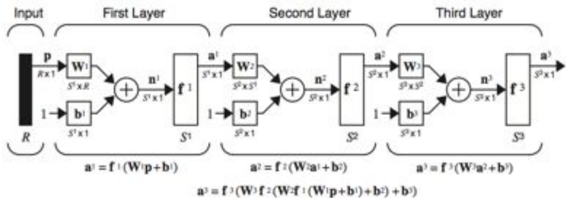
Figure 10.8: Three-layer network
