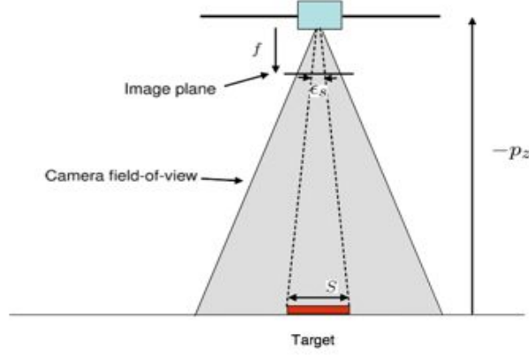
Figure 8.1: The size of the target is S in meters and the size of the target in the image plane is denoted by \epsilon_s in pixels. The focal length is f and the height above the target is -p_z
