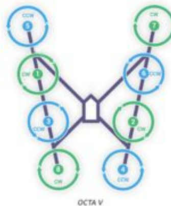
Figure 1.17: Octorotor V design configuration
