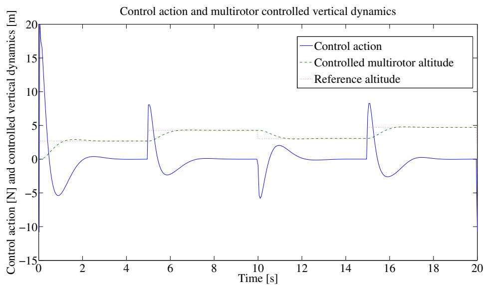
Figure 10.21: Control action and multirotor controlled vertical dynamics
