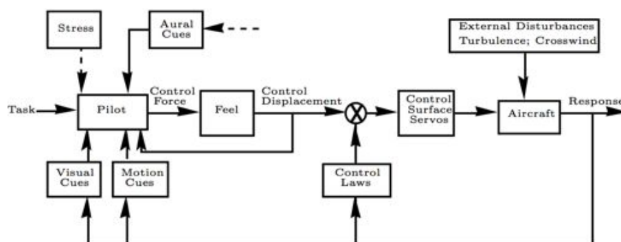
Figure 9.7: Pilot-vehicle dynamic system [3]
