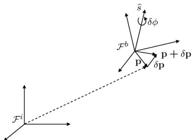
Figure 2.9: Derivation of the equation of Coriolis
