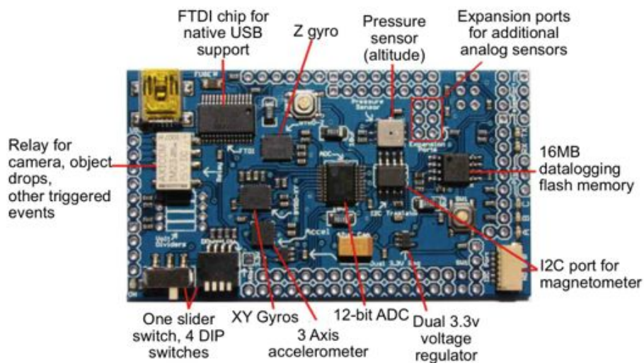
Figure 4.2: The OilPan Inertial Measurement Unit
