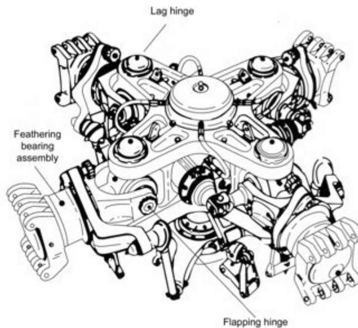
Figure 1.1: Full-scale helicopter swashplate [1]
