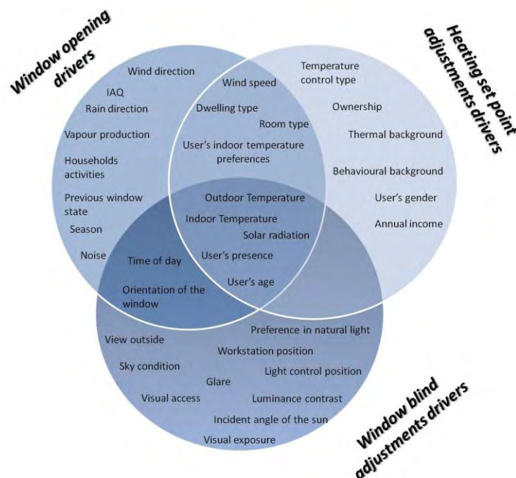
Figure 2. Predominant occupant behaviour drivers for window opening, heating set-point and window blind adjustments.
