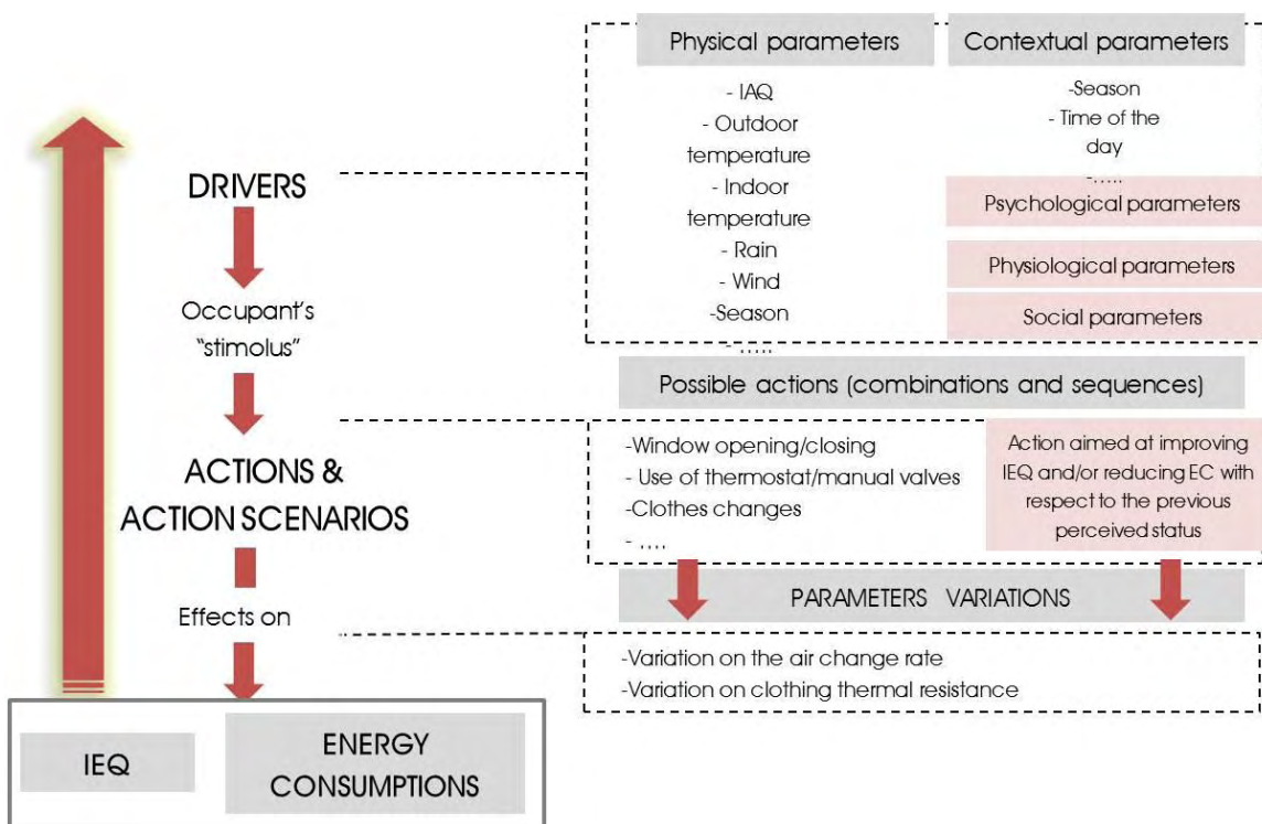
Figure 1. Flux diagram: from drivers to energy consumption and indoor environment.
