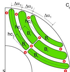
Figure 1. Example of rotor geometry with 3 layers: the \Delta\alpha_j angles define the layer angular positions, hc_j are the layer heights and B_r defines the PM grade. The red circles stand for the point where the eddy-current loss is calculated.
