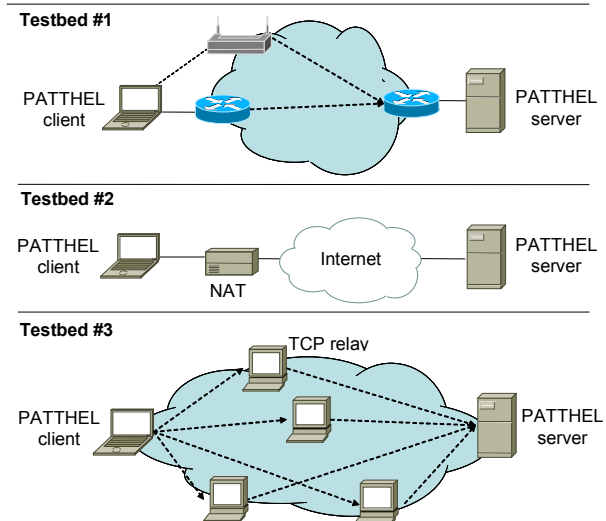
Figure 4. Testbeds.
