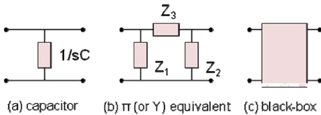
Figure 8 Simplified equivalent structures assumed for the VDD-VSS structure. (a) capacitor; (b) lumped 2-port equivalent ( Z_1 = 1/sC_1 , Z_2 = 1/sC_2 and Z_3 = R_S ) and (c) black-box element defined by a real rational scattering matrix.
