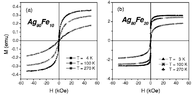
FIG. 1. Isothermal magnetization curves of \text{Ag}_{90}\text{Fe}_{10} and \text{Ag}_{80}\text{Fe}_{20} -cosputtered films at selected temperatures.
