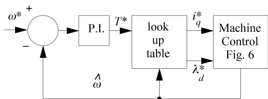
Fig. 10. General control scheme.
