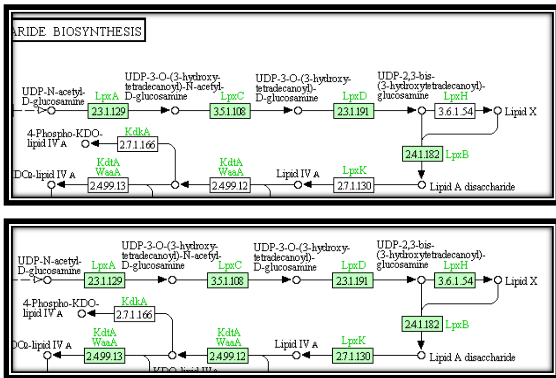
Figure 3. M. ruber (Top) and E. coli Lipopolysaccharide biosynthesis pathway (Bottom). Enzymes are shown in green text with their corresponding E.C. numbers listed below. These images were taken from KEGG and cropped in order to focus on Lipid A disaccharide biosynthesis.
