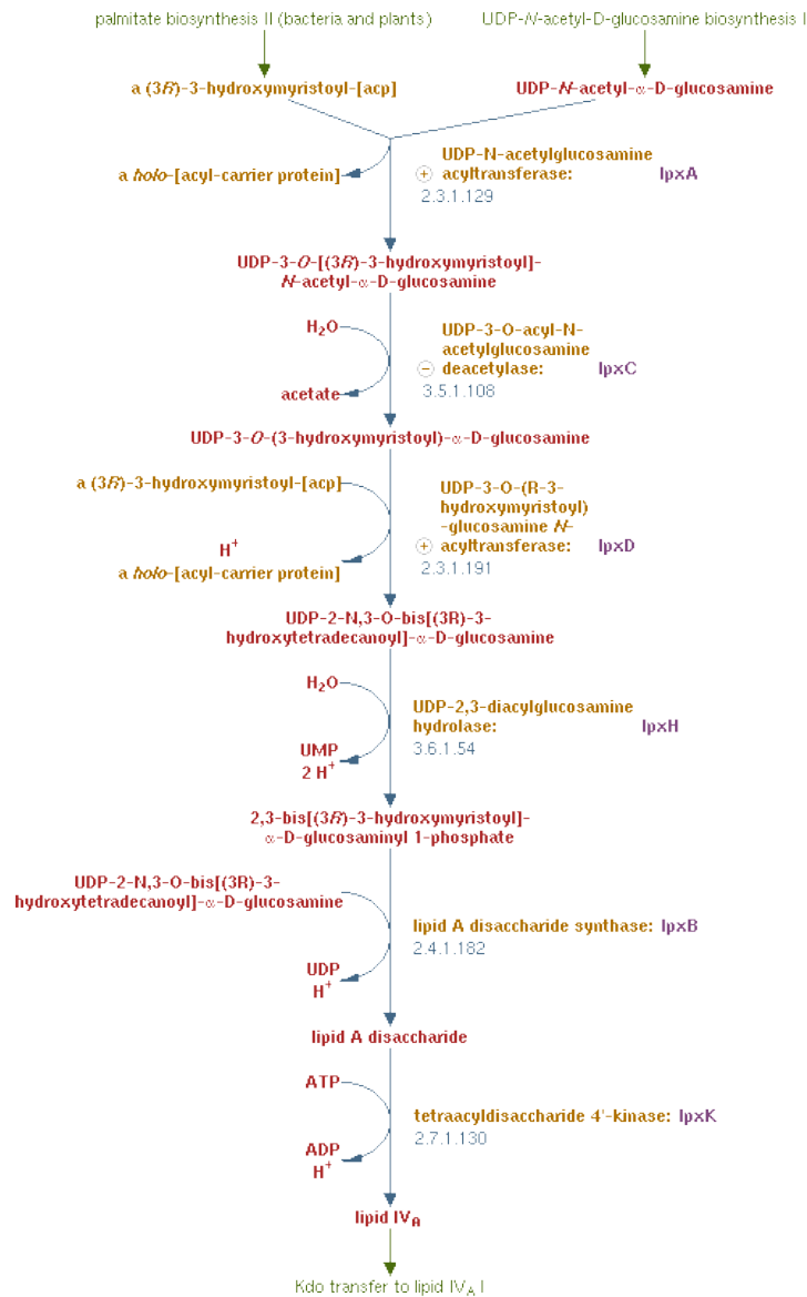
Figure 1. Lipid IV A biosynthesis pathway. The reactants, intermediates, and product are in red and the enzymes are gold with alternate names in purple. Image from MetaCyc.
