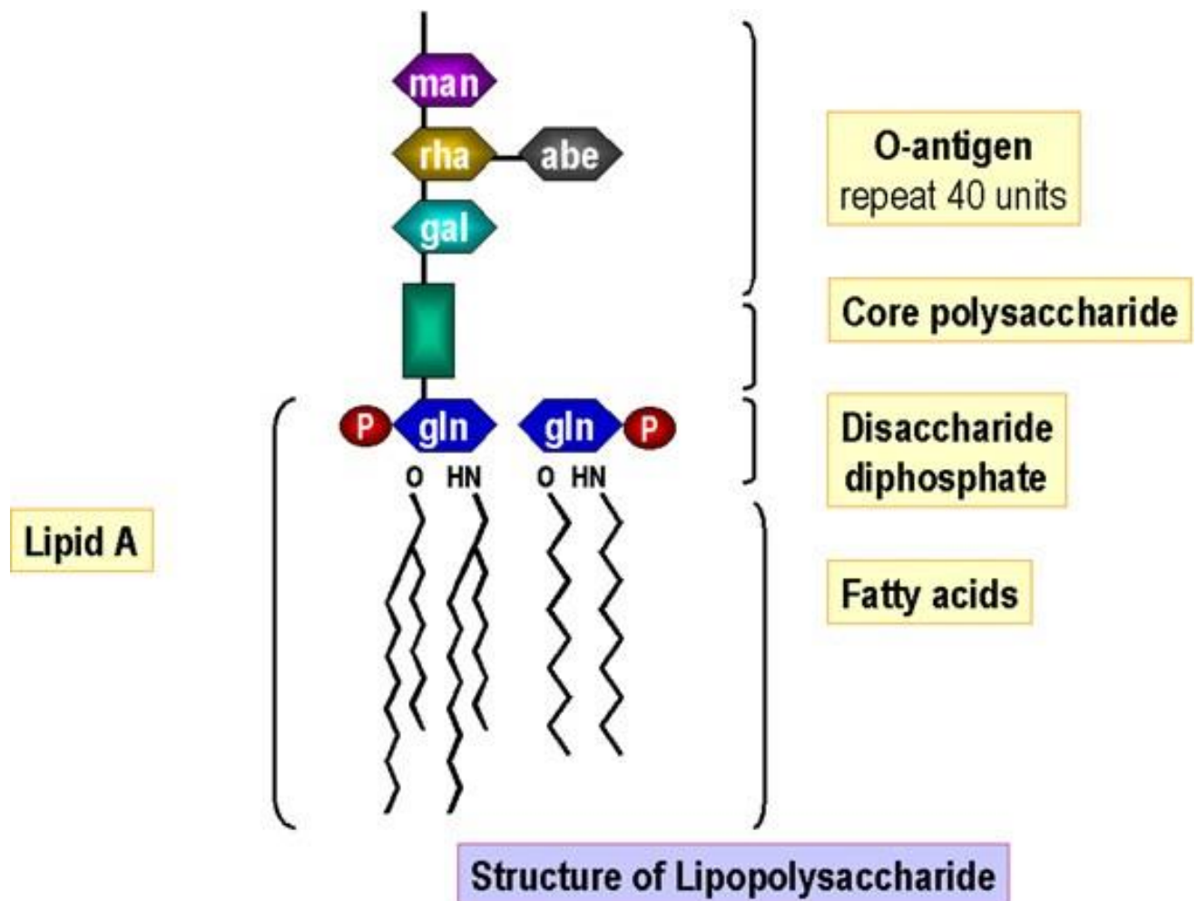
Figure 2. Structure of a Lipopolysaccharide. Lipid A is embedded into the OM of the bacteria because it has multiple hydrophobic fatty acids. Image from: http://i0.wp.com/microbeonline.com/wp-content/uploads/2013/04/lipopolysaccharides.jpg
