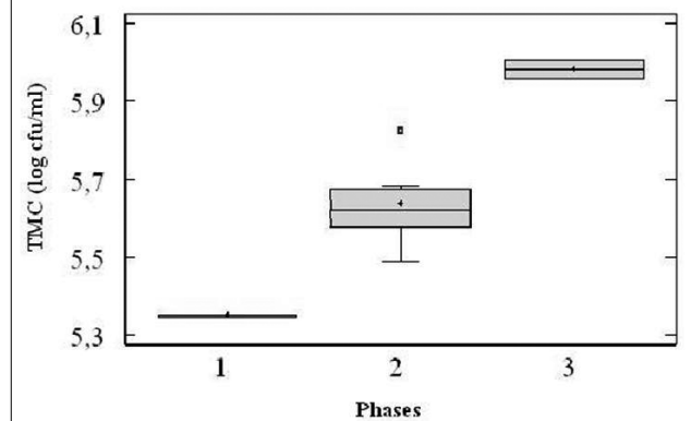
Fig. 5. Box-and-Wisker Plots of TMC in the different phases of Artemia production. Phases: 1 = Start Enrichment; 2 = End Enrichment;; 3 = Manteinance.
