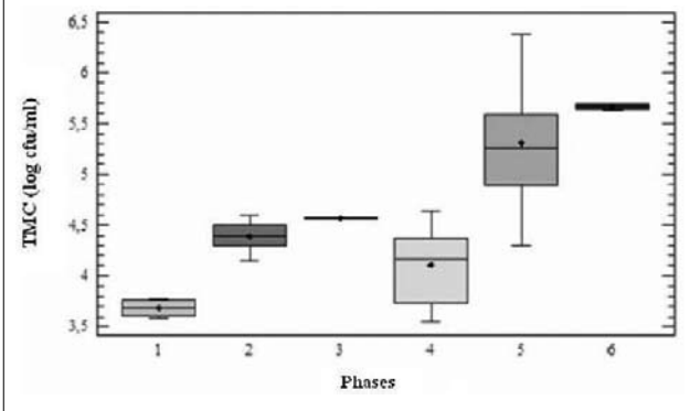
Fig. 3. Box-and-Wisker Plots of TMC in the different phases of Rotifers production. Phases: 1 = Inoculation; 2 = Release; 3 = Culture Start; 4 = Culture End; 5 = Enrichment; 6 = Manteinance.
