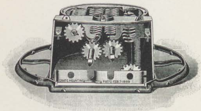
TRIANGULAR GRATE
