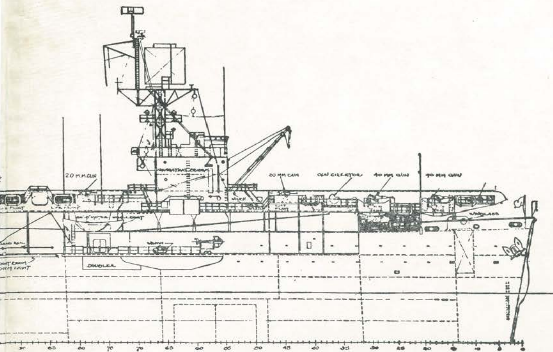
CVE 70 OUTBOARD PROFILE
