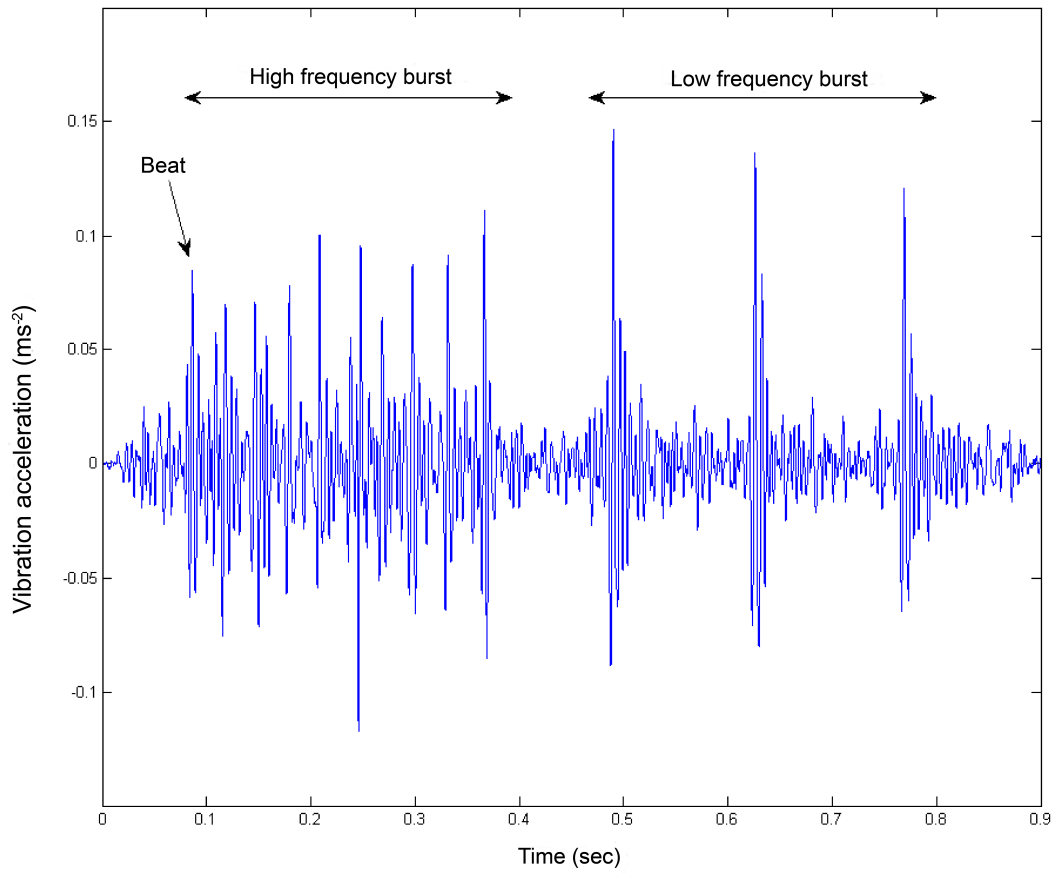
Fig. 2. Example of vibratory behaviour showing the typical structure of the vibratory movements of workers and soldiers of Reticulitermes flavipes . The complex vibrations occurred at two distinct frequencies, described as high (31 Hz) and low (7.4 Hz) frequency bursts.
