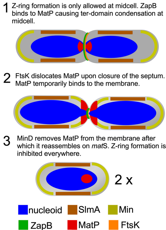
FIG 5 Hypothetical model of the MatP dissociation from the matS sites and its binding to the cytoplasmic membrane. In step 1, ZapB is binding MatP at midcell, causing the 23 matS sites to cluster and ensuring that the terminus remains at midcell. Z-ring formation is inhibited at the old poles by the Min system and in the cylindrical part of the cell close to the bulk of the nucleoid, but not in the Ter domain, by the nucleoid occlusion protein SlmA. The brown bar indicates the nucleoid occlusion by SlmA, not the binding of SlmA to the nucleoid. In step 2, the nucleoids are segregating and MatP is pulled away from ZapB. At the same time, the terminus is bound by FtsK that displaces MatP from matS sites by translocation of the DNA near the terminus, which allows final segregation of the nucleoids into the daughter cells. In step 3, MinD removes MatP from the membrane, after which it reassembles on matS . Z-ring formation is inhibited everywhere by the Min system and the nucleoid occlusion protein SlmA.
